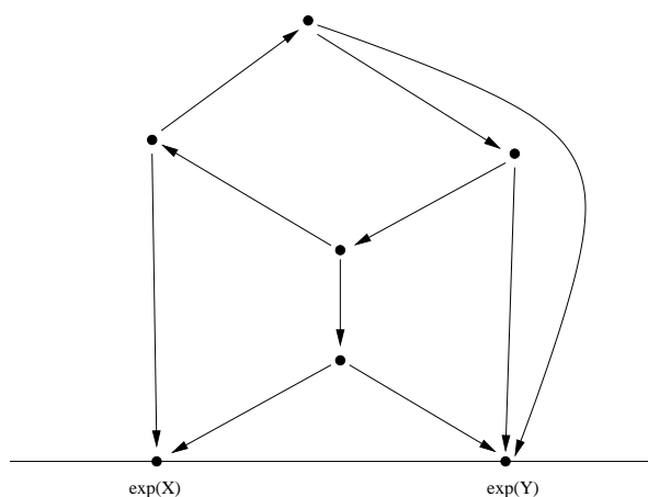
FIGURE 3. Graphe de type roue et de symbole \Gamma(X, Y) = \text{tr}_{\mathfrak{g}}(\text{ad}X\text{ad}[X, Y]\text{ad}Y\text{ad}Y) .
