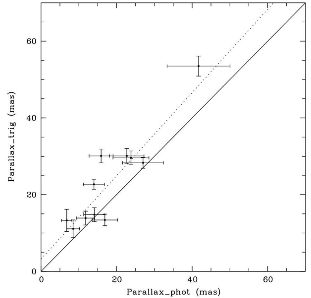
Fig. 2. Comparison of parallaxes derived in this work with photometric parallaxes from OHDHS (errors are assumed 20% for \pi_{\text{phot}} ). Parameters of a weighted linear regression (diagonal line) between both types of parallaxes are \pi = 1.08\pi_{\text{phot}} + 3.21 [mas] with a reduced \chi^2 = 8.06 . The photometric distances are systematically larger than the astrometric ones.
