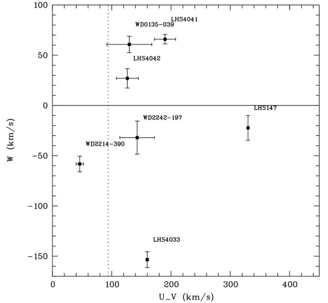
Fig. 6. Component of motion perpendicular to the Galactic plane ( W ) as function of \sqrt{U^2 + V^2} . Only objects with parallax measured at the 4 \sigma level or better and with available radial velocity (Salim et al. 2004) are plotted. The vertical line is the OHDHS \sqrt{U^2 + V^2} = 94 km/s cut.
