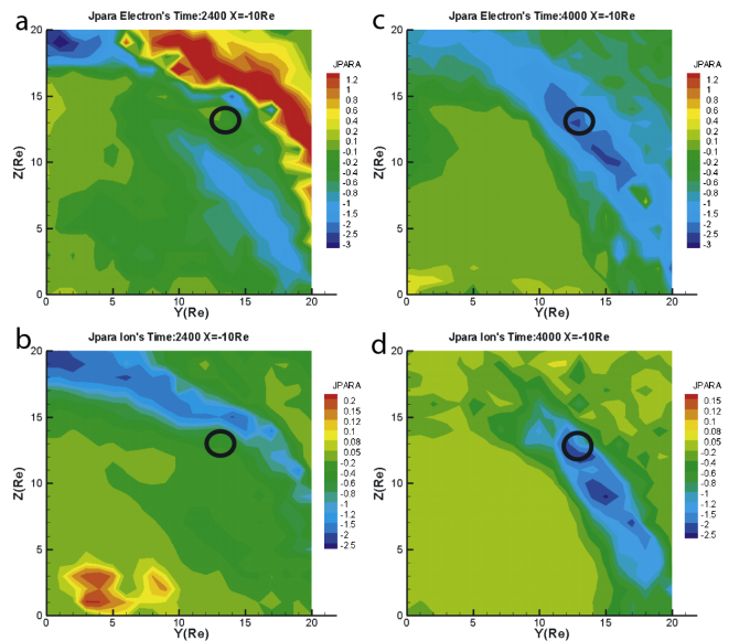
Figure 4. Parallel (a) electron and (b) ion flux components (isocolors) in our global 3DEMP simulation at \tilde{t} = 2400\Delta\tilde{t} at x = -10RE . Parallel (c) electron and (d) ion flux components (isocolors) at \tilde{t} = 4000\Delta\tilde{t} .
