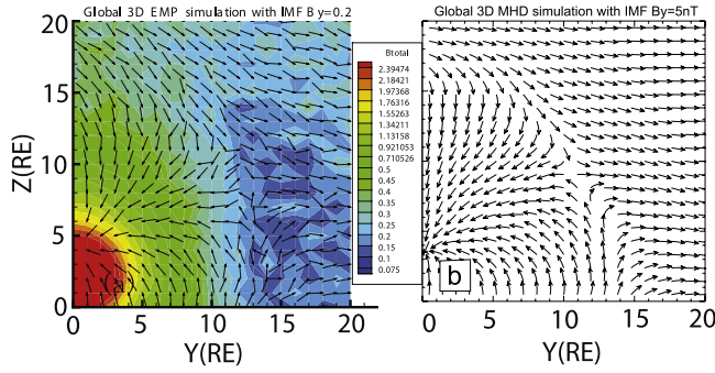
Figure 1. Y - Z sectional slices of magnetic field vector with duskward IMF B_y ( >0 ) near magnetotail at x = -5RE . Results are issued from (a) our global 3D EMP simulation with IMF B_y = 0.2 at \tilde{t} = 4000\Delta\tilde{t} (isocolors correspond to total B field values), and (b) global 3D MHD simulation with IMF B_y = 5nT [White et al. , 1998].
