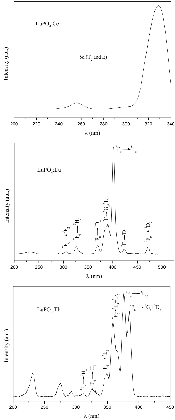
Figure 5: Excitation spectra of LuPO 4 :Ce 3+ (0.5%), LuPO 4 :Eu 3+ (10%) and LuPO 4 :Tb 3+ (5%) recorded at room temperature and respectively at \lambda_{em} = 360 nm, \lambda_{em} = 592 nm and \lambda_{em} = 541 nm
