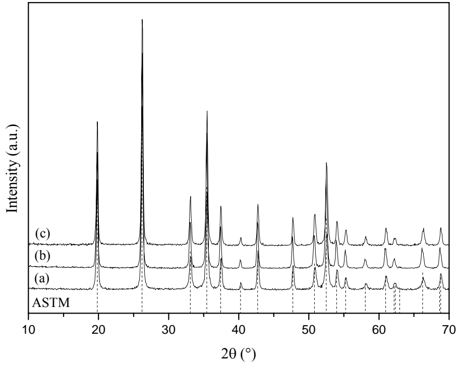
Figure 1: X-Ray diffraction patterns recorded for (a) \text{LuPO}_4:\text{Ce}^{3+} (1%), (b) \text{LuPO}_4:\text{Eu}^{3+} (10%) and (c) \text{LuPO}_4:\text{Tb}^{3+} (5%) with the corresponding reference patterns (dotted lines)
