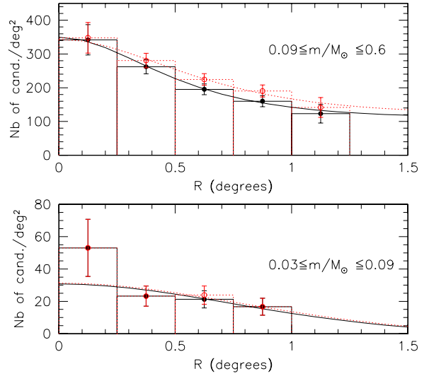
Fig. 12. Radial distribution of the low mass star candidates (upper panel) and the VLM & BD probable cluster members (lower panel). The cluster center has been estimated using the isodensity contours (Fig. 11). In both cases, the filled dots and solid histogram represent the 100 Myr sample while the empty dots and dashed line histogram correspond to the 150 Myr sample. The best \chi^2 fit of a King profile is given for each histogram.
