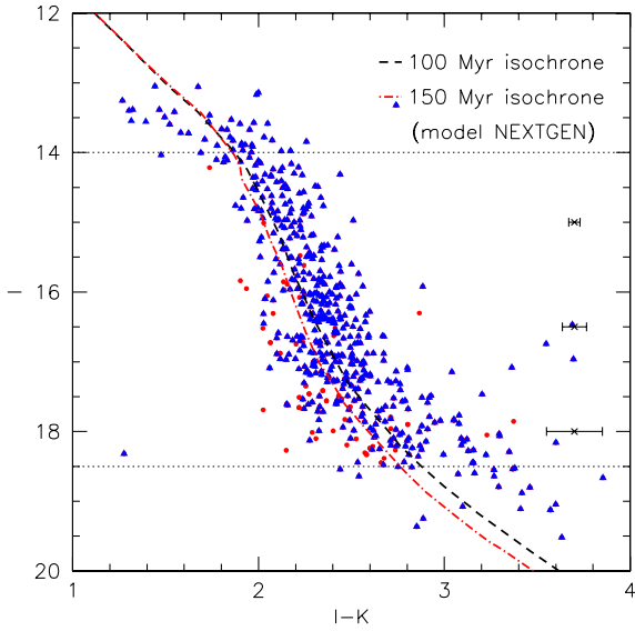
Fig. 3. (I, I - K) colour-magnitude diagram for all the optically selected candidates which have a 2MASS counterpart. The dashed and dot-dashed line are the 100 Myr and 150 Myr isochrones from the NEXTGEN models of Baraffe et al. (1998) shifted to the Blanco 1 distance. The symbols are the same as in Figure 2.
