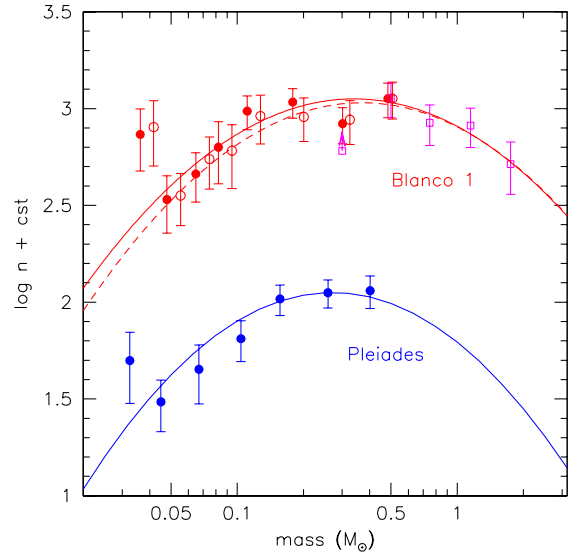
Fig. 14. The mass function of Blanco 1, from low mass brown dwarfs to the most massive stars, fitted by a log-normal distribution (solid line and dashed line for the 100 Myr and 150 Myr sample respectively). The large filled (100 Myr sample) and open (150 Myr sample) dots are our data points completed in the more massive star domain by Pillitteri et al. (2003) data (open squares). The Pleiades mass function (data points and log-normal fit from Moraux et al. 2003) is shown for comparison (see Section 4).
