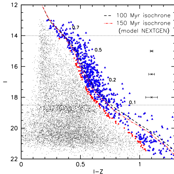
Fig. 2. (I, I - z) colour-magnitude diagram for the short exposures of the optical survey. The dashed (dot-dashed) line is the 100 Myr (resp. 150 Myr) isochrone from the NEXTGEN models of Baraffe et al. (1998) shifted to the Blanco 1 distance. The triangles and large dots correspond to our photometric selection of cluster member candidates for both ages (see text). Typical error bars are shown on the right side.
