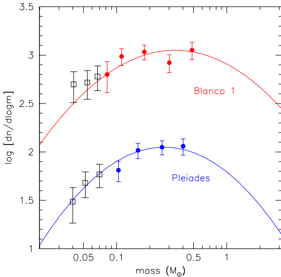
Fig. 15. The Blanco 1 and Pleiades mass function obtained after applying the empirical magnitude-mass relation given by Dobbie et al. (2002). The open squares are the data points which have been modified while the filled circles are the data points which did not change. The log-normal fit for each cluster is shown as a solid line.
