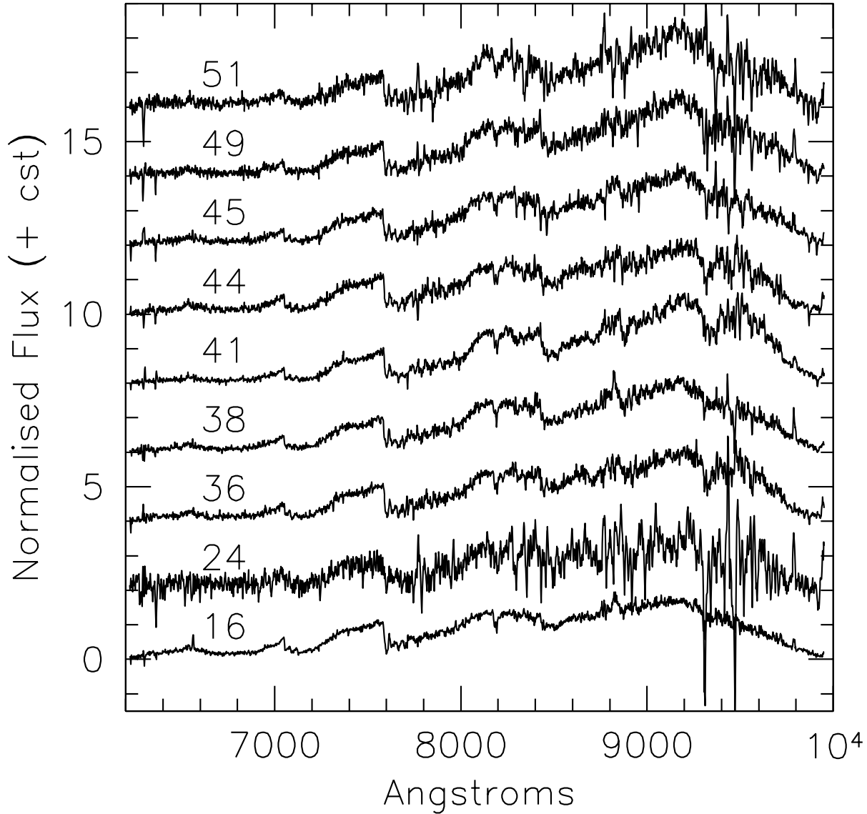
Fig. 8. LRIS spectra of CFHT-BL VLM candidates.
