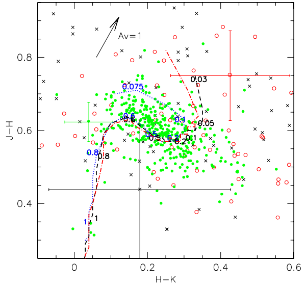
Fig. 4. (J - H, H - K) colour-colour diagram of all the low mass star candidates with a 2MASS counterpart. The different symbols correspond to different flags in the 2MASS catalog, i.e. different photometric accuracy (dots = flag A, open circles = flag B, crosses = flag C). A typical error bar is represented for each symbol. The 100 Myr, 150 Myr and 5 Gyr (corresponding to the field dwarf locus) isochrones are shown as a dashed, dot-dashed and a dotted line respectively and are labelled with mass. The reddening vector is also shown. All candidates are located on or close to the isochrones – within the error bars – indicating that there is little extinction and that they all have near-infrared colours consistent with M-dwarf spectral type.
