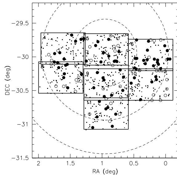
Fig. 1. Area of the sky covered by the CFHT 1999 and 2000 Blanco 1 surveys. Each rectangle corresponds to one CFH12K field (the coordinates are given in Table 1). The small cross in the middle represents the nominal cluster center and the dashed circles have a radius of 0.5, 1 and 1.5 degrees respectively. Small dots show the location of low mass star candidates selected from the short exposures. Very low mass star and brown dwarf candidates selected from the long exposures are shown as large dots if confirmed by infrared photometry and/or optical spectroscopy (open circles if ruled out).
