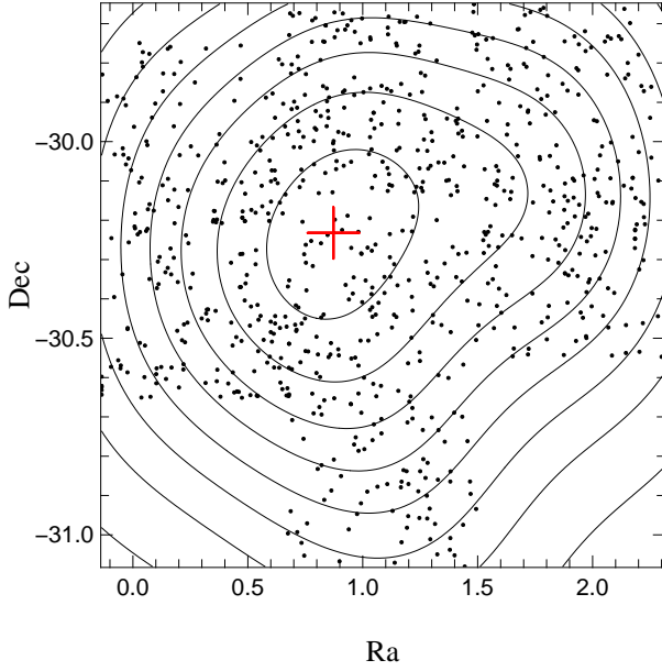
Fig. 11. Spatial distribution of all the cluster member candidates detected in the short exposures and selected from the 150 Myr isochrone. Contours of isodensity are drawn. The cross represents the peak of density and is taken as the cluster center whose coordinates are (0.87,-30.2) in degrees.
