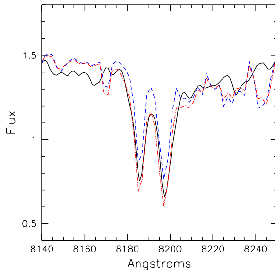
Fig. 10. Upper panel: Comparison of the Na I doublet profile of BL-29 (solid line) with two synthetic spectra of similar T_{eff} for \log g = 4.5 (dashed line) and 5.0 (dot-dashed line). Lower panel: Same as before but for GJ-866 which is an older field dwarf having the same spectral type than BL-29 (M6).
