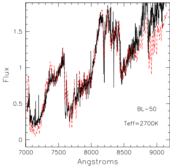
Fig. 9. Spectrum of BL-50 (solid line) fitted by a synthetic spectrum (dashed line) from the DUSTY models of Allard et al. (2001). The best fit gives T_{eff} = 2700\text{K} , which is in agreement with the M7-M7.5 spectral type we find using the PC3 index or the comparison to spectroscopic standards.
