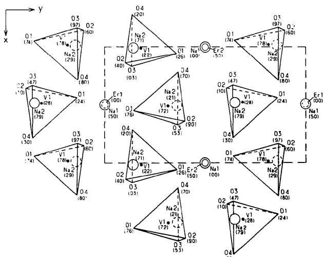
Fig. 1. Projection of the \alpha\text{-Na}_3\text{Er}(\text{VO}_4)_2 structure on the (001) plane.
