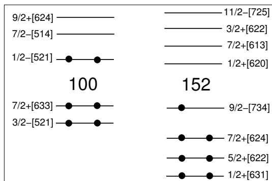
Fig. 6. Schematic representation of the available proton (left) and neutron (right) single-particle levels calculated in reference [1]. The filled circles illustrate the filling of the orbitals in the ground state of ^{253}\text{No} .
