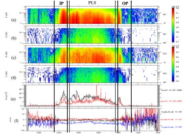
Fig. 2. CIS data: (a)-(b) distribution of H^+ and He^+ for C1; (c)-(d) same data for C3; (e) H^+ density for C1 and C3; (f) H^+ velocity V_H for C1 in GSE coordinates.
