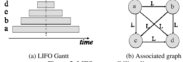
(a) LIFO Gantt (b) Associated graph
