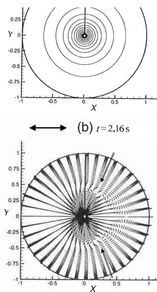
FIG. 12. 2D numerical simulation of the vibrational convection in an ideal gas at T = 300 \text{ K} \approx T_c and the same vibration conditions as in Fig. 11. (a) Temperature profile. (b) Onset of two convection rolls (arrows). Two symmetrical rolls will grow at the next period, forming in average four counter-rotative rolls.
