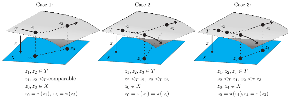
FIGURE 1. Irreducible cycles
