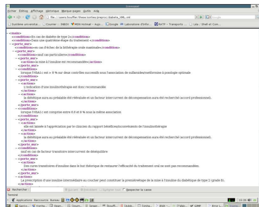
Figures A2 and A3. The original text, and the XML GEM template instantiated from the text
