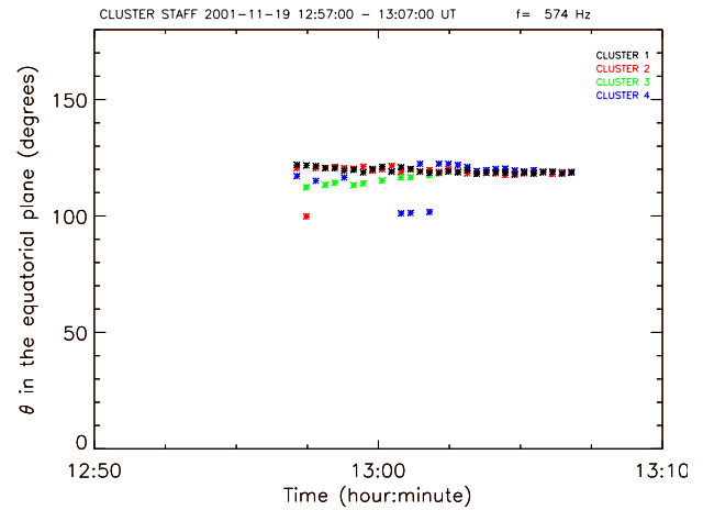
Fig. 4. Representation of the polar angle \theta in the equatorial plane given by the ray tracing software as a function of time (it is the same time interval as Fig. 3) for each SC at 574 Hz.
