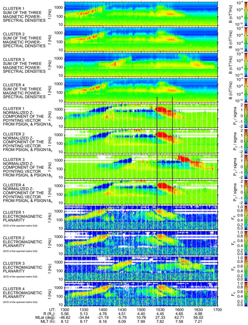
Fig. 6. Same as Fig. 1 but for the chorus event recorded on 7 November 2001 between 13:00 and 17:00 UT.
