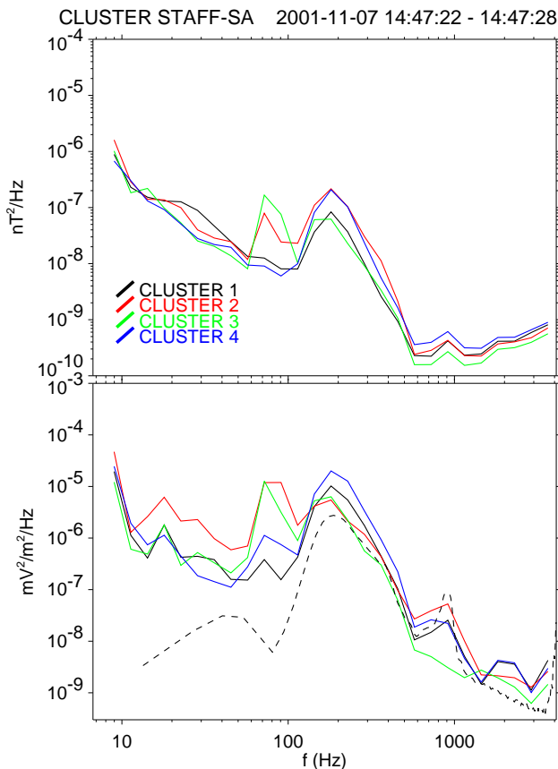
Fig. 11. Magnetic (top) and electric (bottom) power spectral densities recorded by STAFF-SA for each SC as a function of frequency during the same time interval as Fig. 10. The dashed line in the bottom panel is from WBD.
