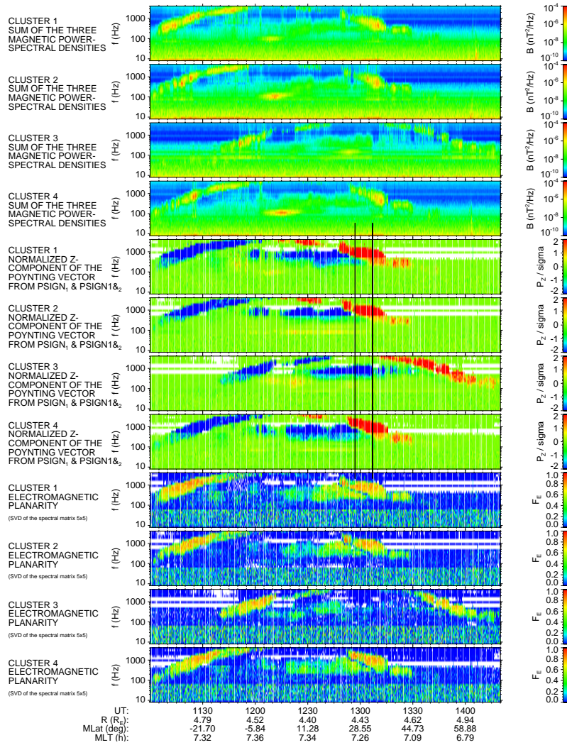
Fig. 1. Chorus event recorded on 19 November 2001 between 11:00 and 14:20 UT. From the top to the bottom, spectrogram of magnetic power spectral densities, z-component of the Poynting vector and degree of planar polarization are represented for the four SC, respectively. Values are color-coded according to the scales on the right. The two vertical lines indicate the time interval where the ray tracing is done.
