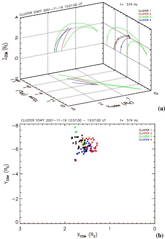
Fig. 3. Results of the ray tracing performed on 19 November 2001 at a frequency equal to 574 Hz. (a) 2-D projections of one 3-D trace are represented for each SC according to their allocated colors at 13:01 UT. The arrows in the plane YZ indicate the real trajectory of the waves. The stars indicate the positions of the SC. (b) Location of the equator crossing in the equatorial plane for each SC between 12:57 and 13:07 UT.
