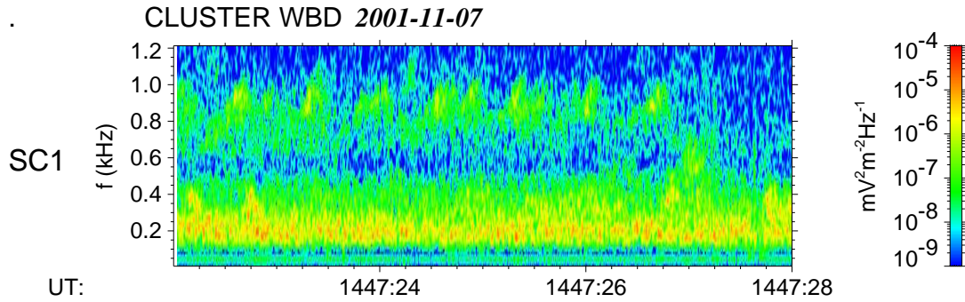
Fig. 10. Spectrogram of one electric component recorded by WBD on 7 November 2001 between 14:47:22 and 14:47:28 UT for SC1.
