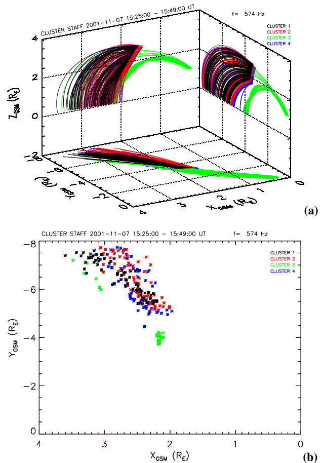
Fig. 8. Results of the ray tracing performed on 7 November 2001 between 15:25 and 15:49 UT at a frequency equal to 574 Hz. (a) In comparison to Fig. 3a, here all the rays are represented during the given time interval. (b) Location of the equator crossing in the equatorial plane for each SC.
