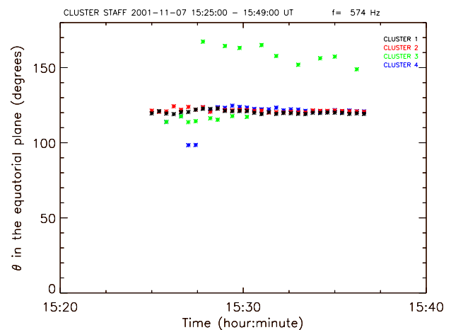
Fig. 9. Same as Fig. 4 but for 7 November 2001 between 15:25 and 15:49 UT.
