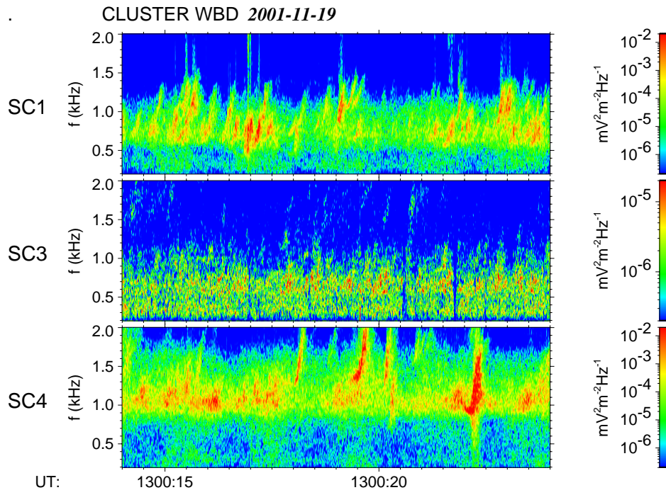
Fig. 5. Spectrograms of one electric component recorded by WBD on 19 November 2001 between 13:00:14 and 13:00:24 UT for SC1 (top), SC3 (middle) and SC4 (bottom).
