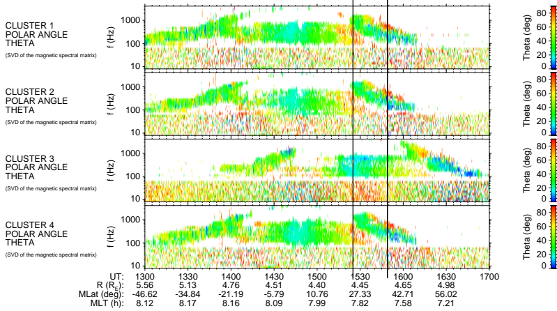
Fig. 7. Same as Fig. 2 but for 7 November 2001.
