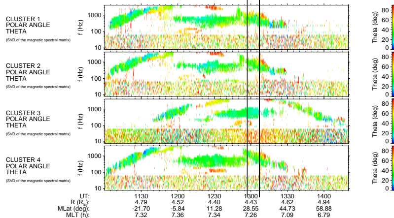
Fig. 2. Spectrograms of the wave normal angles for the event of Fig. 1 for the four SC. Values are color-coded according to the scales on the right. The two vertical lines indicate the time interval where the ray tracing is done.
