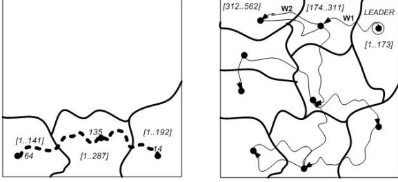
Fig. 2. After the paths construction (dashed lines) between clusters, the global initialization is just executed by means of the gossiping algorithm performed via these paths.
