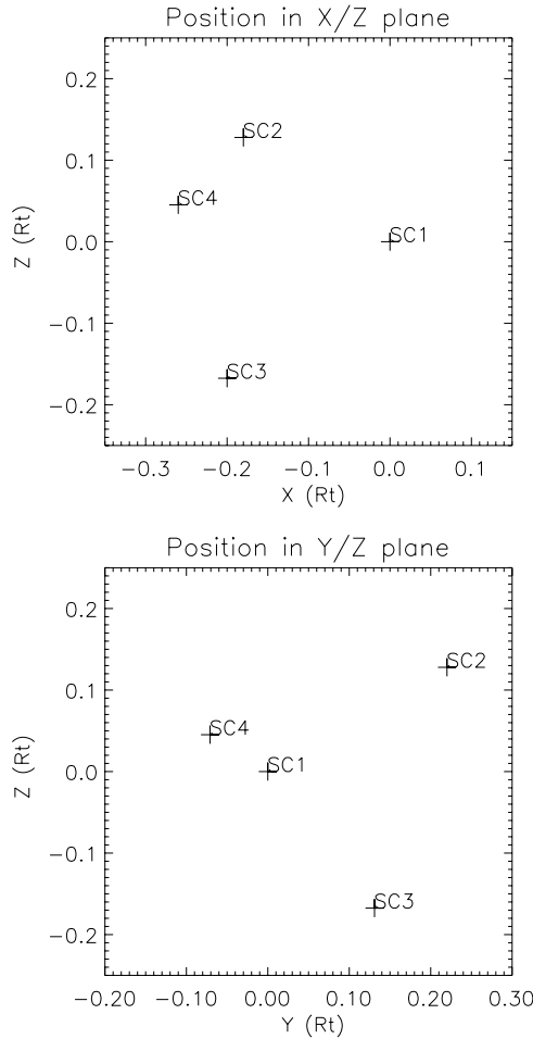
Figure 5. Relative position of the four spacecraft in the GSM frame.
