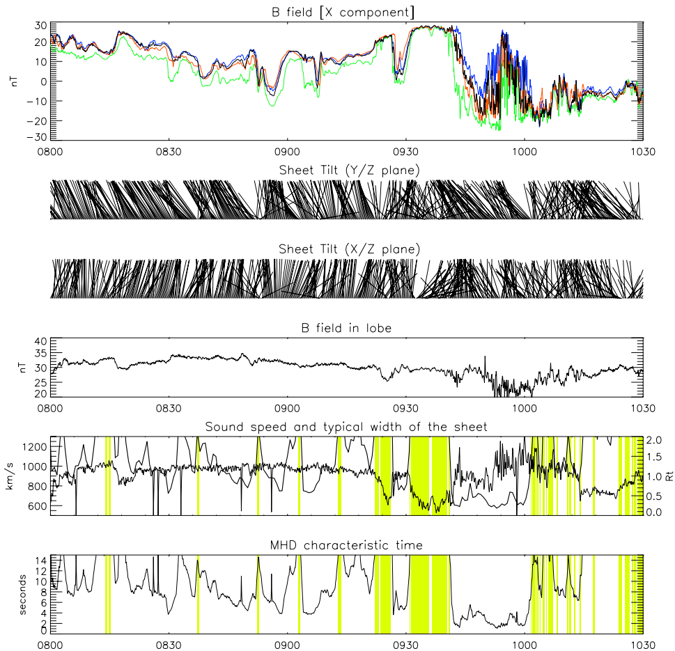
Figure 6. Geometrical and physical parameters of the plasma sheet. Panel 1: B_x component (SC1 in blue, SC2 in red, SC3 in green and SC4 in black), Panels 2 and 3: projection of the normal vector in plane Y/Z and X/Z , Panel 4: magnetic field in lobe, Panel 5: sound speed and half-thickness of the sheet (thick line), Panel 6: MHD characteristic time \tau = a/v_s . The yellow zones correspond to periods of poor estimates of the sheet thickness (Cluster in the lobes).
