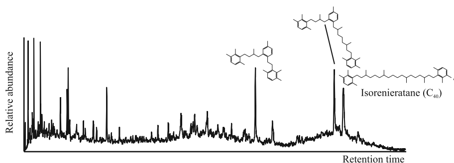
Figure 4. Mass chromatogram ( m/z 133 + 134) of the apolar fraction of a representative (HTM 102, 805.74 m) black shale from the ANDRA core section. Major isorenieratene derivatives are indicated.
