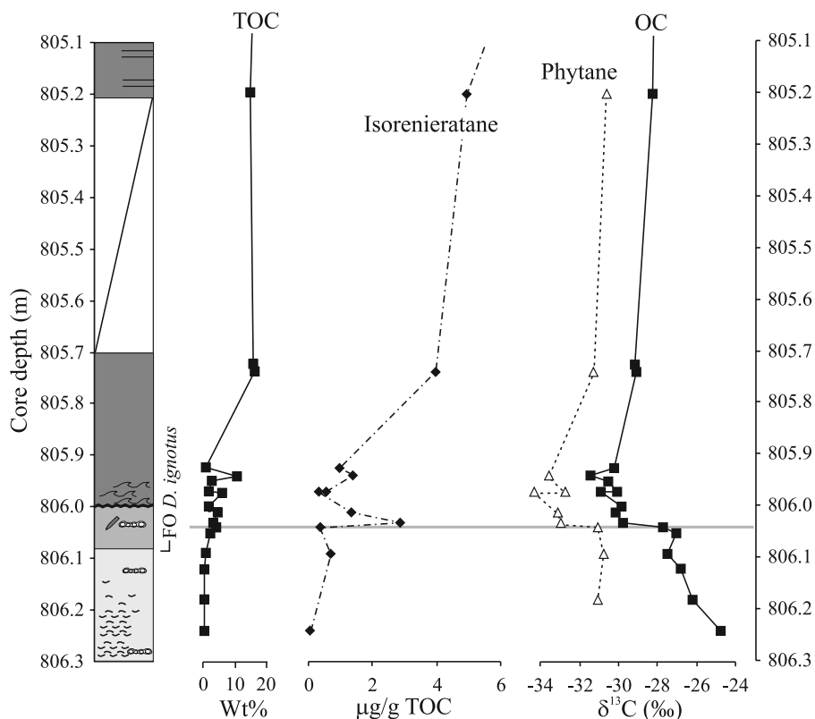
Figure 3. Detailed view of the negative \delta^{13}\text{C} excursion at the onset of the organic carbon rich sediments, accompanied by corresponding TOC and isorenieratane abundances. Legend as in Figure 2.
