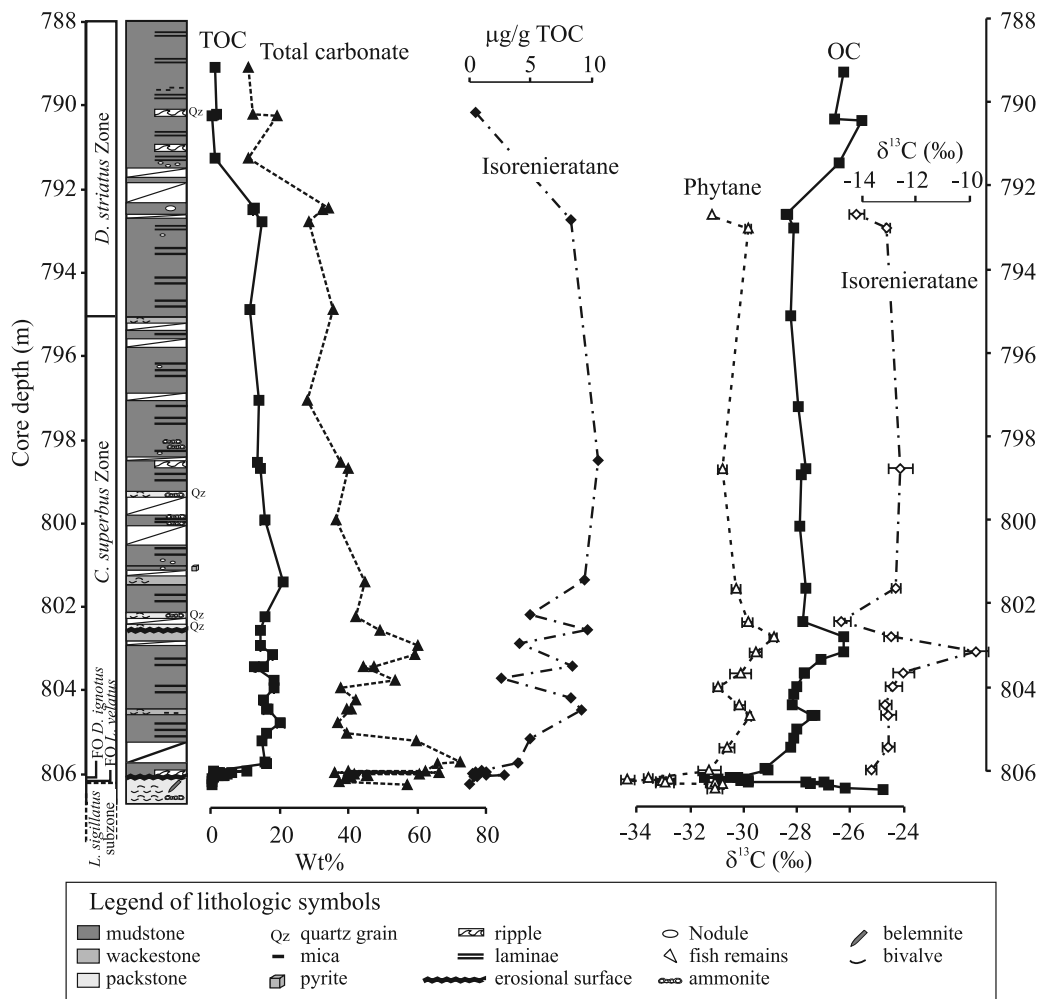
Figure 2. Lithostratigraphy with nanofossil zones of the ANDRA Core HTM 102 at Cirfontaine-en-Ornois (Lorraine, France). Also shown are stratigraphic records for TOC and bulk carbonate content (in wt% of sediment), isorenieratane abundances and stable carbon isotope ratio of TOC, phytane and isorenieratane. FO: first occurrence.
