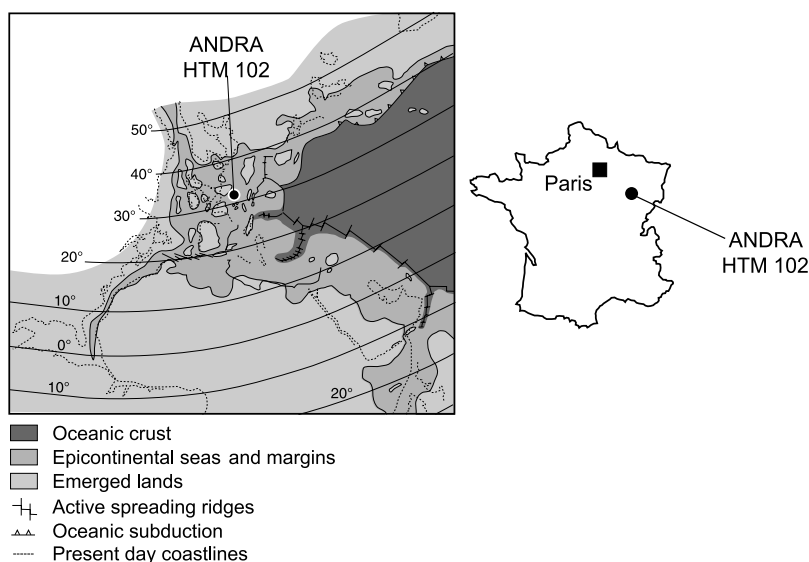
Figure 1. Paleogeographical frame of the drill core site [Mattioli et al. , 2004] and the location of the drill site in France (inset).
