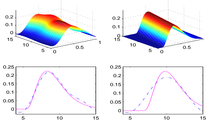
FIGURE 1. Plots of the estimated (top-left) with trigonometric basis and the true (top right) conditional density and y \mapsto \pi(x, y) (full line), \tilde{\pi}(x, y) (dashed dotted line) for x = 0.15 (bottom-left) and x = 0.90 (bottom-right) with n = 2000 observations in Example 2 and without censoring.
