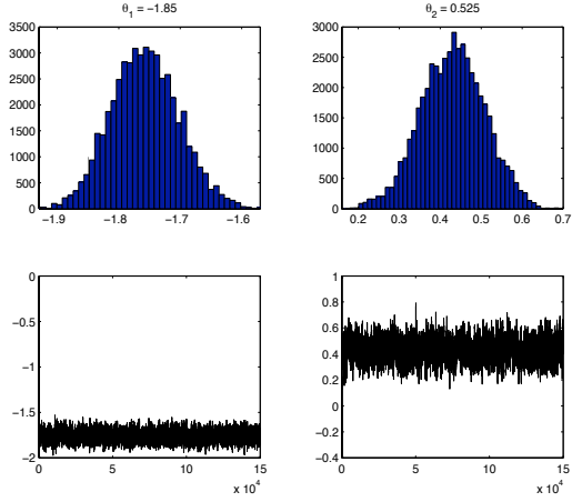
Figure 3. Histograms of the posterior distribution (on \theta_1 and \theta_2 ) and Markov chains associated, 150000 iterations.
