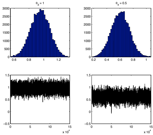
Figure 4. Histograms of the posterior distribution (on \theta_3 and \theta_4 ) and Markov chains associated, 150000 iterations.
