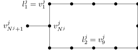
Figure 4: The gadget H(e_j) for k = 4 and d^j = 2 .
