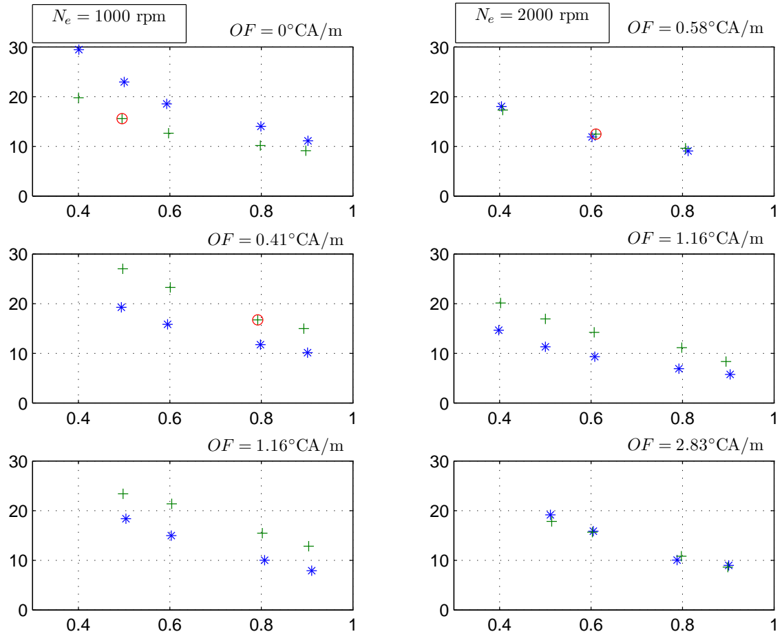
Figure 1. Residual gas mass fraction \chi_{res} in percentages as a function of the ratio p_{man}/p_{exh} for two engine speeds N_e and different overlapping factors OF . The 26 experimental data are represented by plus signs (+) with a superposed circle ( \oplus ) for the 3 points retained as training samples. The 26 simulation data appear as asterisks (*).
