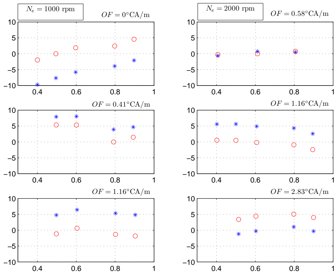
Figure 2. Errors on the experimental data (training and test samples) for the prior model (*) and the OD-model (o) trained with only three samples ( N = 3 ).
