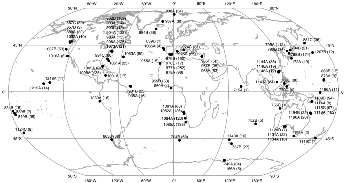
Figure 3. Location of the ODP sites where thermal conductivity measurements \lambda and well logs could be combined. Number of data { \lambda , well logs} per well in parentheses.
