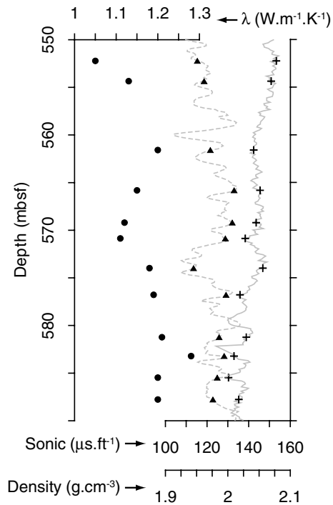
Figure 1. Example of thermal conductivity measurements (circles) associated with values of two well logs at corresponding depths (sonic: crosses; density: triangles). Well logs are also shown (sonic: solid line; density: dashed line). The same procedure is applied to the other well logs (see text). Data are taken from a section of ODP site 1109D.
