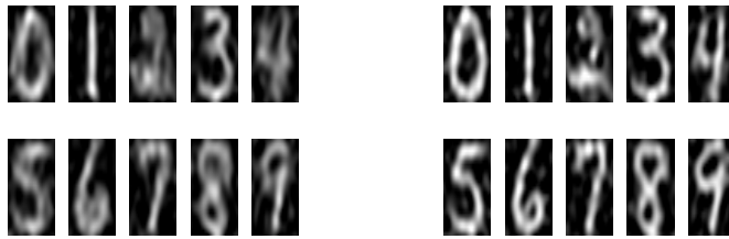
FIG. 5.12. Estimated prototypes in a noisy setting \sigma^2 = 2 : Left: with the mode approximation algorithm. Right: with the SAEM-MCMC coupling procedure.
