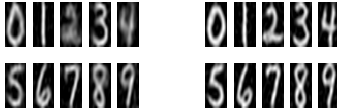
FIG. 5.11. Estimated prototypes in a noisy setting \sigma^2 = 1 : Left: with the mode approximation algorithm. Right: with the SAEM-MCMC coupling procedure.
