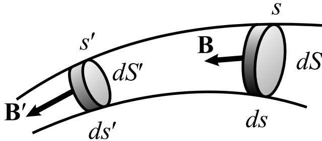
Figure 2. Diagram of an elementary flux tube. Each position along the tube is described by the curvilinear abscissa s , \mathbf{B} is the magnetic field, dS the section of the flux tube, and ds an elementary movement along the tube. Two distinct positions are displayed here for abscissa s and s' .
