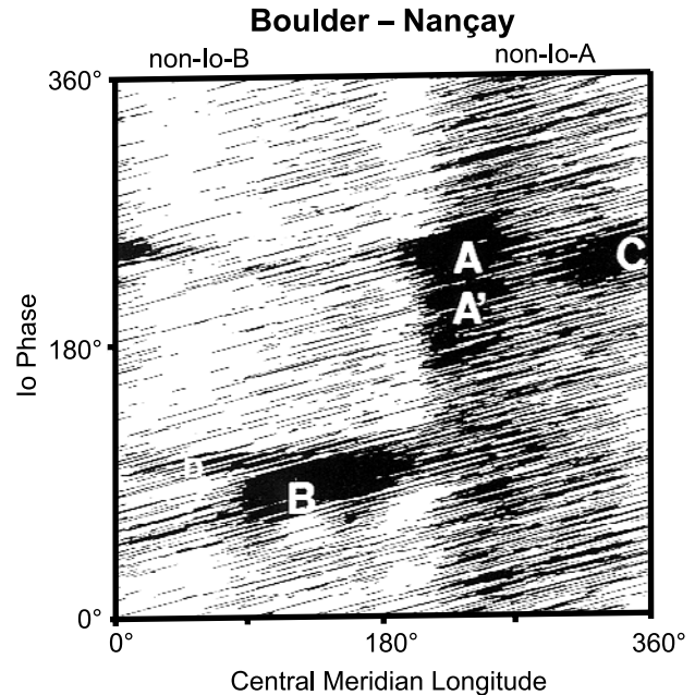
Figure 1. Occurrence probability of jovian decameter radio emissions (as observed by ground-based radio stations) versus system III longitude (CML) and Io phase ( \Phi_{10} ) [after Genova et al. , 1989, and references therein].
