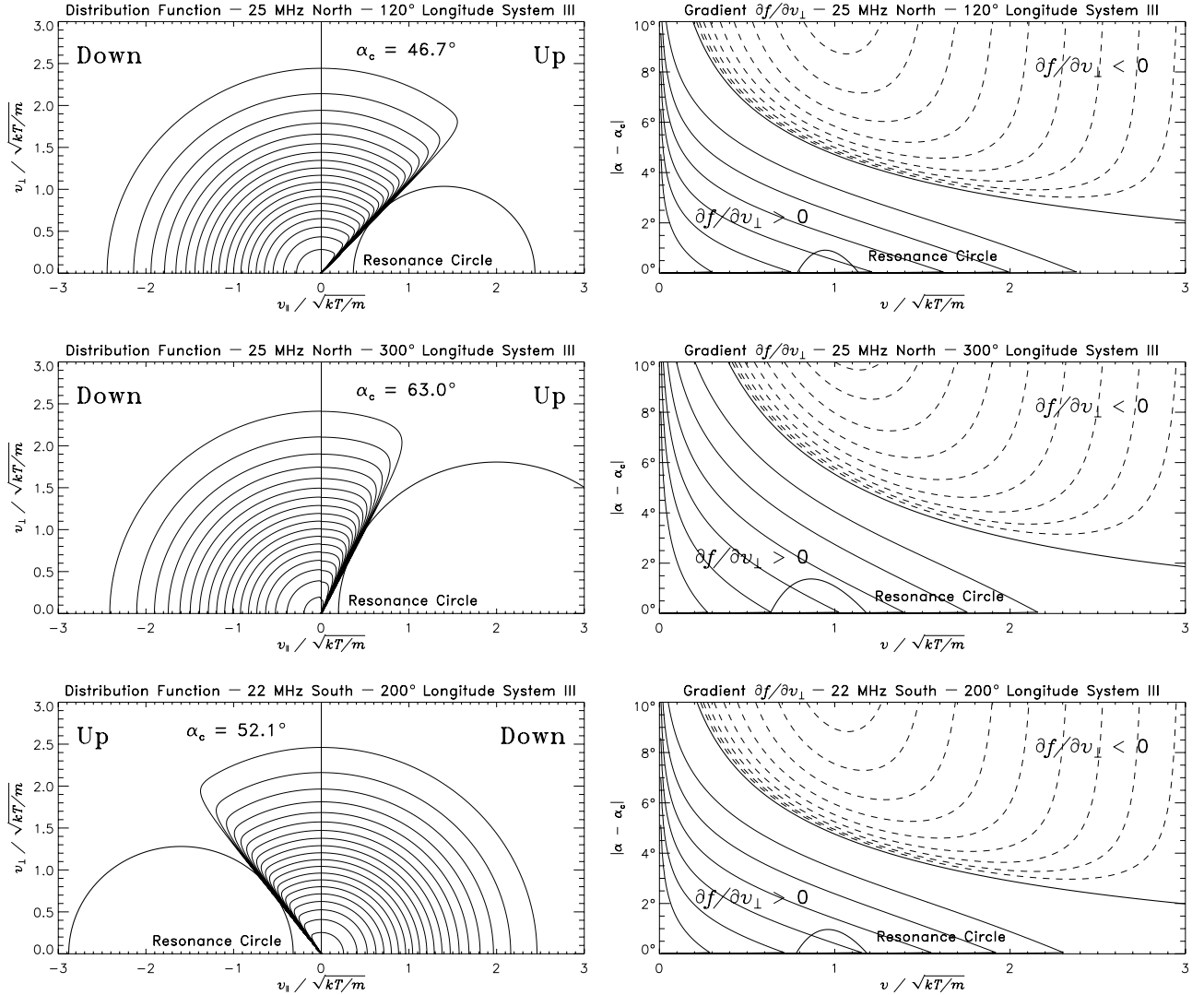
Figure 5. Left panels show contours of the electron distribution function f at the point of the magnetic field line where the gyrofrequency is 25 MHz (Northern Hemisphere) or 22 MHz (Southern Hemisphere). It is plotted for three different longitudes (of system III): 120^\circ , 300^\circ (north) and 200^\circ (south). Right panels show contours of the perpendicular gradient of the distribution function \partial f / \partial v_\perp near the edge of the loss cone plotted for the same values of gyrofrequencies and longitudes. The loss cone is characterized by its opening angle \alpha_c . The optimum resonance circle defined in subsection 3.7 is also displayed; it is tangential to the edge of the loss cone and only a very small portion of the circle penetrates into the region where \partial f / \partial v_\perp > 0 . In all the plots the velocity is normalized to \sqrt{kT/m} where T is the temperature of the initial Maxwellian distribution function at Io. Here k refers to Boltzmann's constant.
