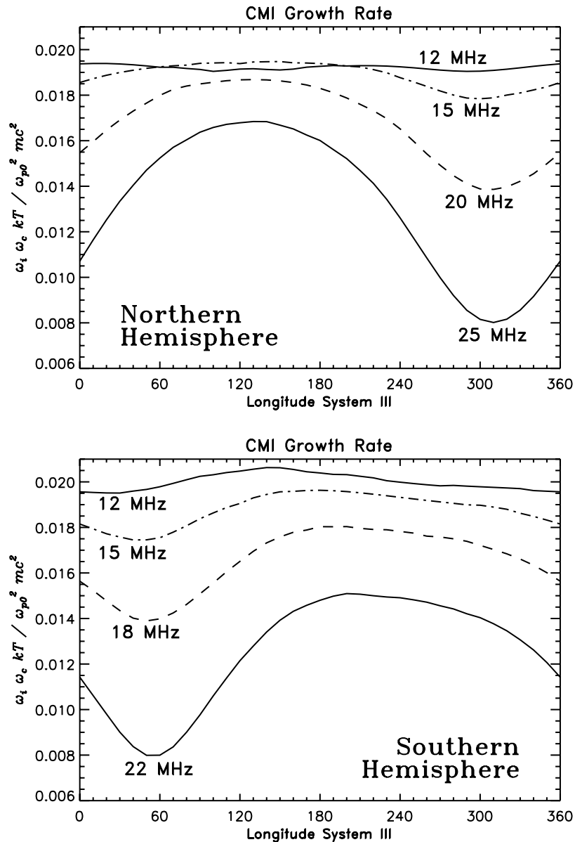
Figure 7. Dimensionless normalized growth rate of the cyclotron maser instability versus jovian longitude (system III), calculated for both hemispheres for four frequencies: 25, 20, 15, 12 MHz (north) or 22, 18, 15, 12 MHz (south). The growth rate \omega_i is normalized to \omega_{p0}^2 mc^2 / \omega_c kT , where \omega_{p0}^2 and T are the plasma frequency and the temperature of the initial electron distribution function at Io and \omega_c the local gyrofrequency.
