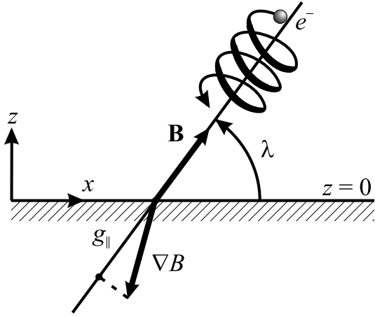
Figure 4. Magnetic field line, in the vicinity of altitude z = 0 in the ionosphere. This part of the line is considered to be rectilinear. Here g_{\parallel} denotes the parallel component of \nabla B , and \lambda is the inclination of \mathbf{B} at altitude z = 0 .
