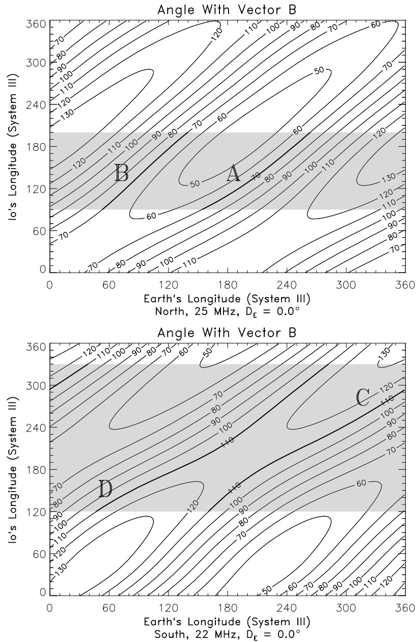
Figure 8. Contours of the angle between the local magnetic field and the direction of the observer (located at Earth). An active longitude range is deduced from the curves in Figure 7 and displayed in gray. The thick segments correspond to emissions with a high probability of occurrence.
