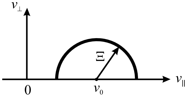
Figure 6. Resonance curve of the cyclotron maser instability in velocity space ( v_{\parallel} , v_{\perp} ): it is approximated to a circle of radius \Xi .
