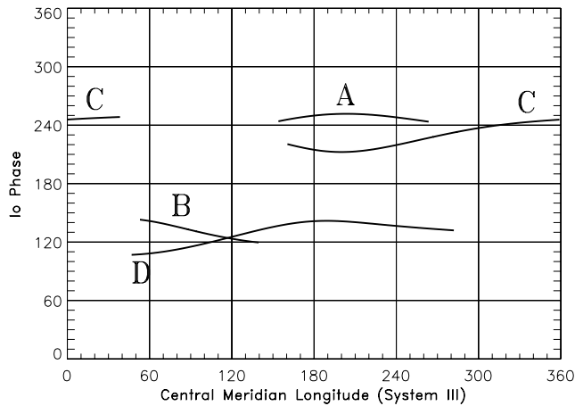
Figure 9. Curves of high occurrence probability versus central meridian longitude and Io phase.
