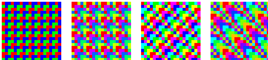
Fig. 1. \Psi(\text{rep}_2(q + \mathbb{N}p)) for p = 3, 5, 6, 8 .
