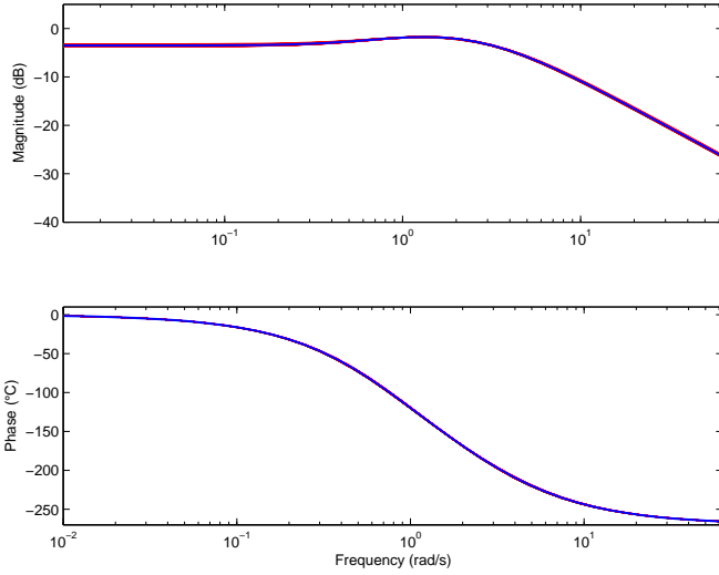
(c) Estimated G_2(s) by SRIVC
