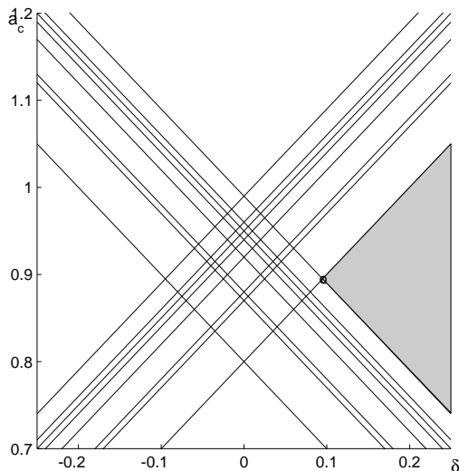
Figure 5: parameter domain in the plan (a_c, \delta)
