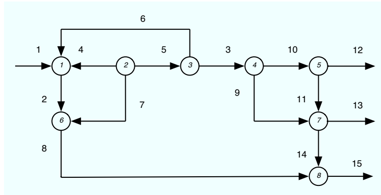
Figure 8: Flowsheet
