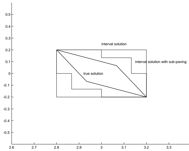
Figure 10: Interval linear system
