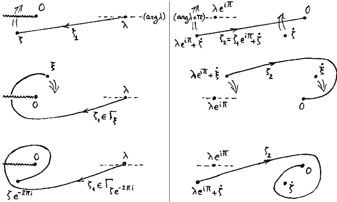
Figure 13: Analytic continuation of \check{\psi}_{3,\lambda} . (Left: three examples of path \Gamma . Right: the corresponding paths followed by \zeta_2 = \zeta_1 e^{i\pi} + \zeta ).
