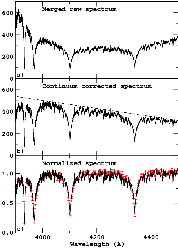
Fig. 1. Normalisation of the spectrum of HD 225125: a) Merged spectrum with incomplete removal of the instrumental signature/response; b) Corrected spectrum and continuum placement (broken line); c) Normalized observed spectrum (black line) compared to the synthetic one (red crosses).
