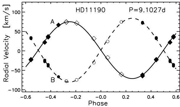
Fig. 10. Radial velocity phase diagram of HD 11190. Full and dashed lines represent the orbital solution assuming a circular orbit. Filled symbols correspond to data collected at NAO Rozhen, unfilled ones to data collected at OHP.
