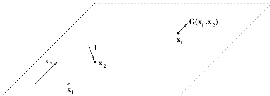
Fig. 1. Green's function.
