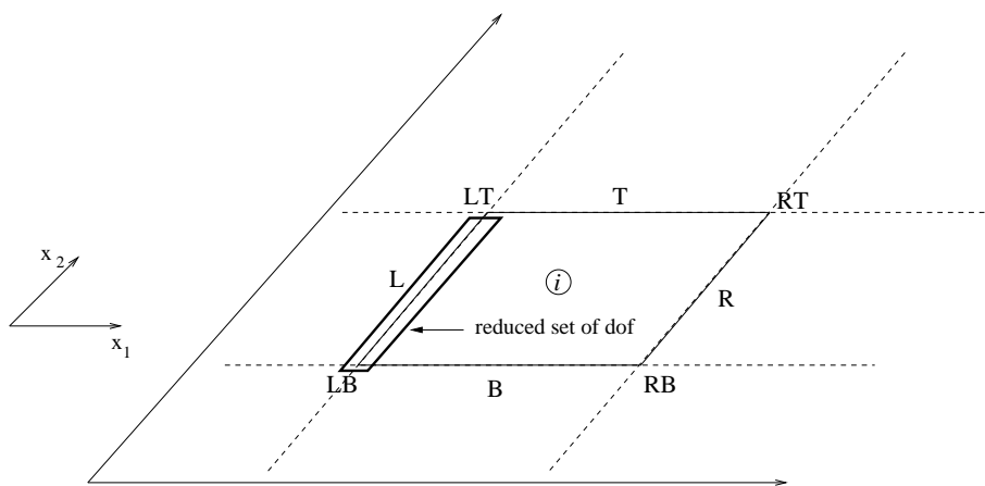
Fig. 4. Reduced set of degrees of freedom.
