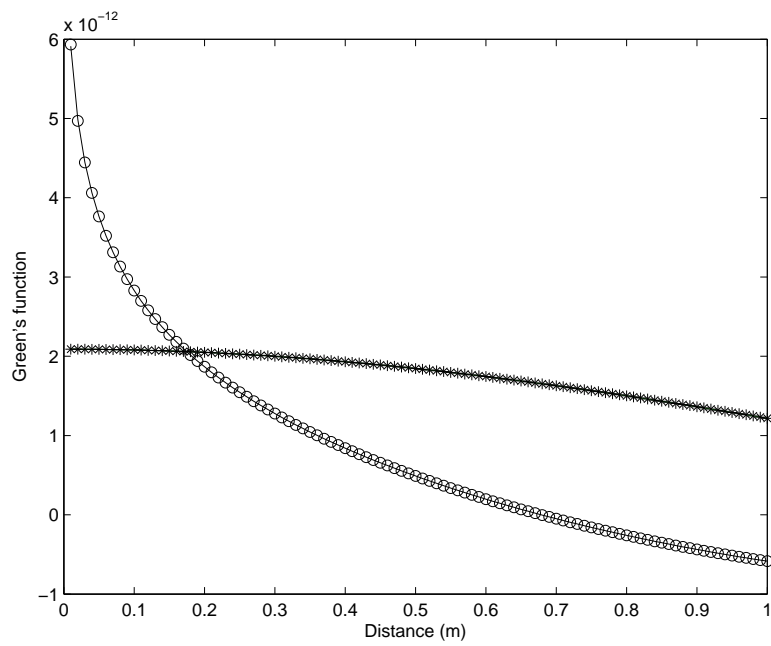
Fig. 13. Comparison of analytical and numerical Green's functions for the two-dimensional elasticity: — real part analytical, - - - imaginary part analytical, x real part numerical, o imaginary part numerical.
