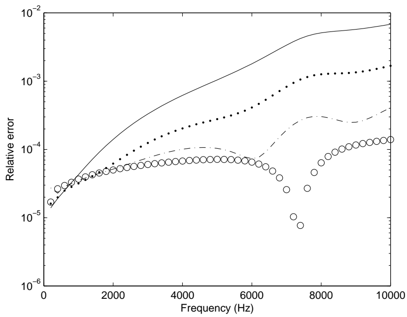
Fig. 11. Error in the Green's function versus the number of elements in the periodic cell for the two-dimensional elasticity: — 1x1 mesh, • 2x2 mesh, -.- 4x4 mesh, o 1x1 mesh of degree 2.
