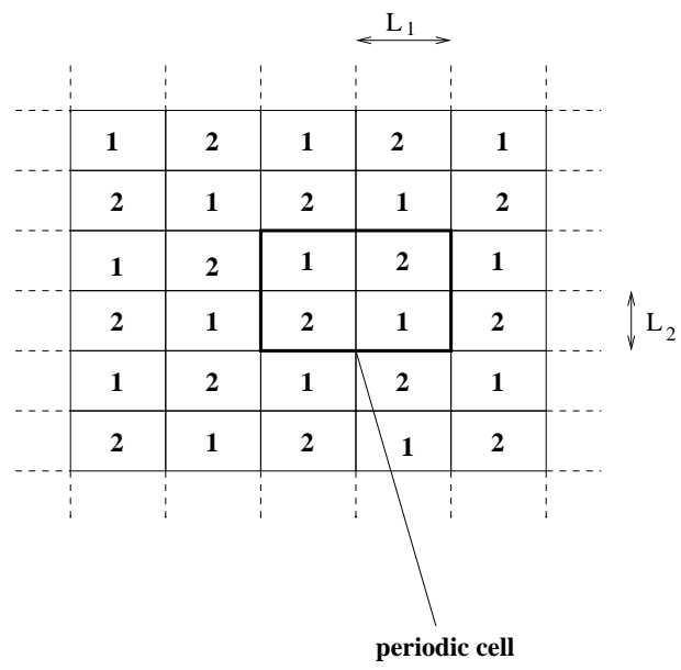
Fig. 14. Network of two materials.
