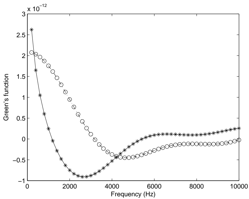
Fig. 10. Comparison of analytical and numerical Green's functions for the two-dimensional elasticity: — real part analytical, - . - . imaginary part analytical, * real part numerical, o imaginary part numerical.
