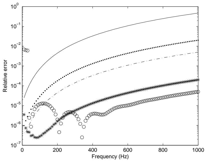
Fig. 9. Error in the Green's function versus the size of the periodic cell for the acoustic case: — a=b=0.05\text{m} , \bullet a=b=0.01\text{m} , -.- a=b=0.005\text{m} , * a=b=0.001\text{m} , \circ a=b=0.0005\text{m} .
