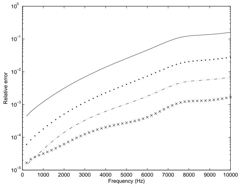
Fig. 12. Error in the Green's function versus the size of the periodic cell for the two-dimensional elasticity: — L_1 = L_2 = 0.05m , • L_1 = L_2 = 0.02m , -.- L_1 = L_2 = 0.01m , × L_1 = L_2 = 0.005m .
