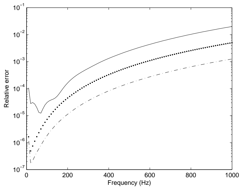
Fig. 8. Error in the Green's function versus the number of elements in the periodic cell for the acoustic case: — 1x1 mesh, • 2x2 mesh, - . - . 4x4 mesh.
