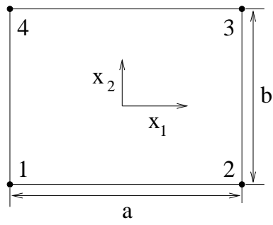
Fig. 6. Four nodes acoustic element.
