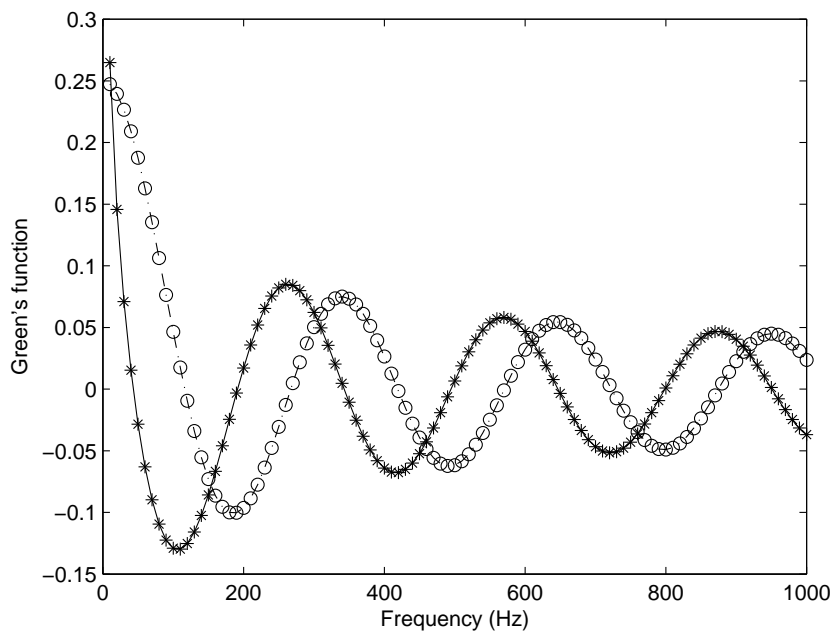
Fig. 7. Comparison of analytical and numerical Green's functions for the acoustic case: ____ real part analytical, -.-. imaginary part analytical, * real part numerical, o imaginary part numerical.
