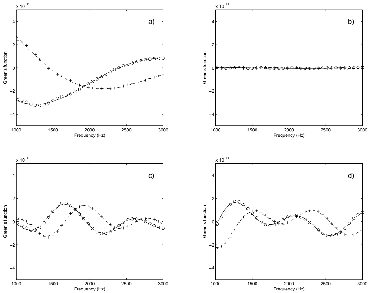
Fig. 15. Comparison of the present method and a full FEM computation for a periodic two materials medium: a) x component of displacement at point (0.25, 0) , b) y component of displacement at point (0.25, 0) , c) x component of displacement at point (0.5, 0.5) , d) y component of displacement at point (0.5, 0.5) , — real part present method, - - . imaginary part present method, \circ real part full FEM, + imaginary part full FEM.
