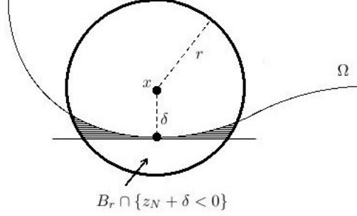
FIGURE 2. Reduction to the flat case
