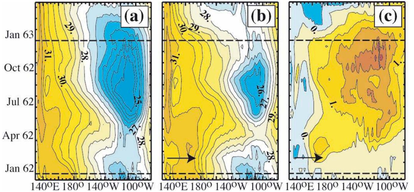
Fig. 6 Time longitude evolution of SST averaged over 2°N–2°S for CREF ensemble mean (a), CWWE ensemble mean (b), and their difference (c). The contour interval is 0.5°C for temperature. The arrow denotes the artificially introduced WWE
