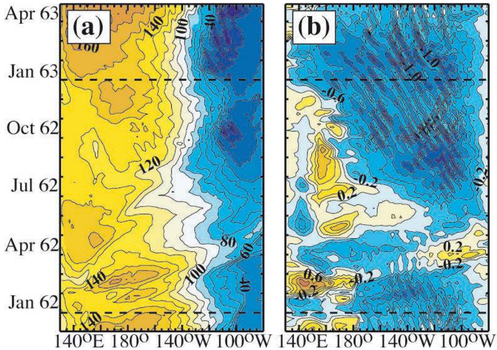
Fig. 13 As Fig. 10 but for MW experiment
