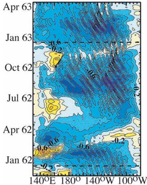
Fig. 15 Time longitude evolution for NC experiment for surface zonal currents averaged between 2°N and 2°S. The contour interval is 0.2 m s -1
