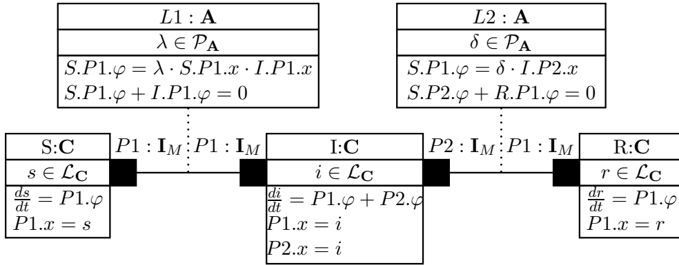
Figure 12: Equivalent multiport diagram of the compartmental network
