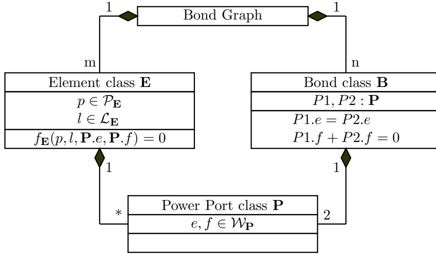
Figure 13: Meta-model of an acausal bond graph
