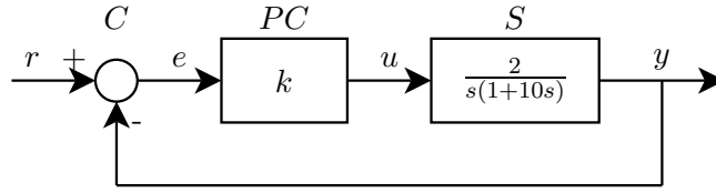
Figure 5: Example of block diagram
