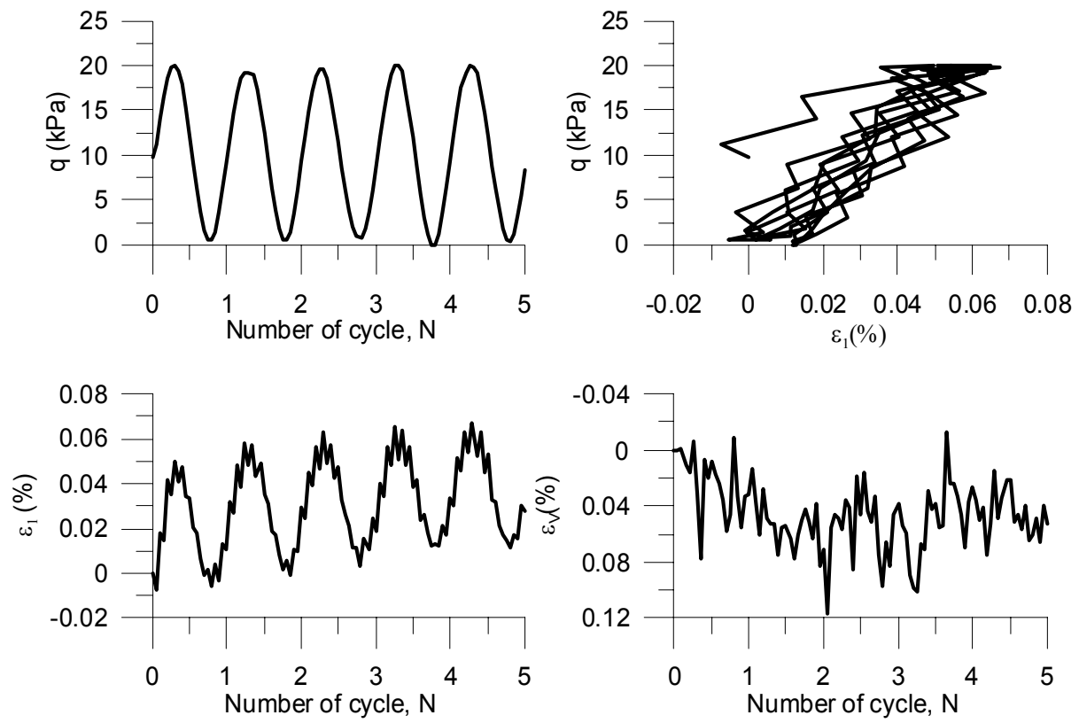
Figure 4. Cyclic triaxial test on unsaturated loess. w = 14\% , f = 0.05\text{ Hz} , \sigma_3 = 25\text{ kPa} . First cycles.
