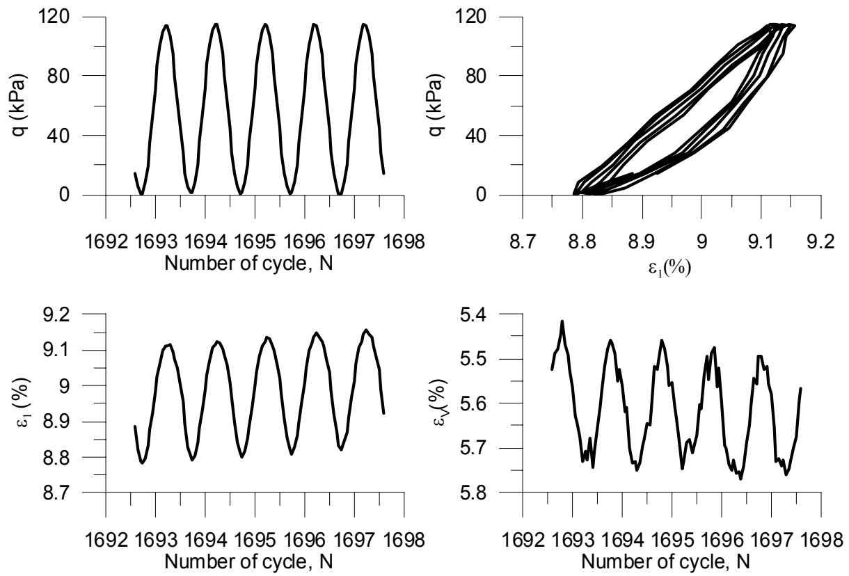
Figure 5. Cyclic triaxial test on unsaturated loess. w = 14\% , f = 0.05 Hz, \sigma_3 = 25 kPa. Last cycles.
