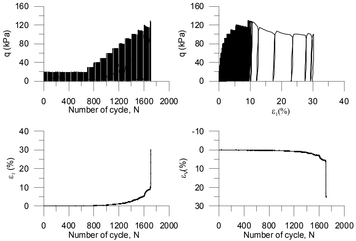
Figure 6. Cyclic triaxial test on unsaturated loess. w = 14\% , f = 0.05\text{ Hz} , \sigma_3 = 25\text{ kPa} .
