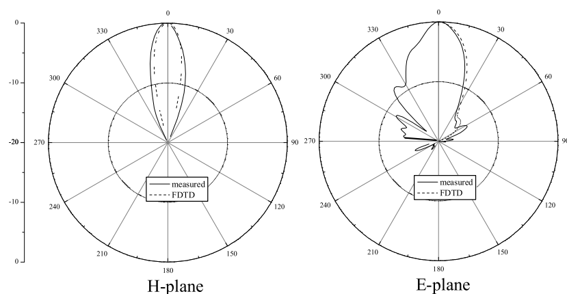
Figure 14. Measured and simulated co-pol radiation patterns in the H-plane and E-plane at 2.63\text{ GHz} .
