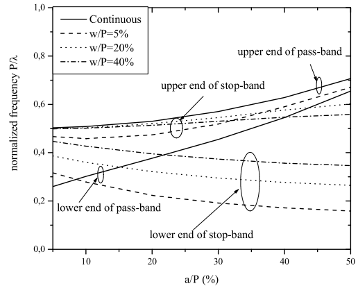
Fig. 5. Two first bands limits for structures with continuous and discontinuous wires ( P_z = P ) versus fill factor a/P , for different widths w/P .
