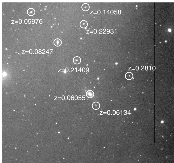
Fig. 2. R band 10.2 \times 9.7 arcmin 2 image of RX J1119 with the known redshifts in the field.
