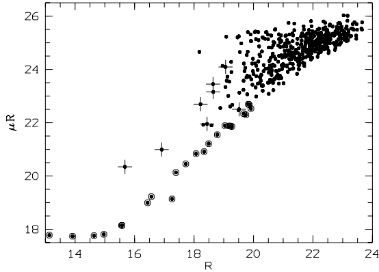
Fig. 4. R central surface brightness versus total R magnitude for the RX J1119 field of view. Objects classified as stars are circled dots. We can see the saturation of the brightest stars. Crossed dots are objects classified as galaxies using spectroscopy.
