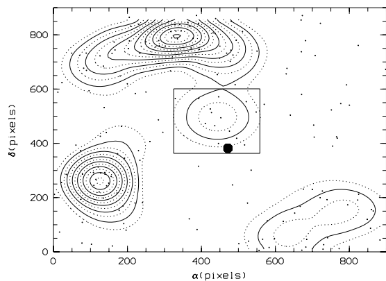
Fig. 6. Adaptive kernel galaxy density map (in pixels) for galaxies inside the blue-delimited area in Fig. 5. The X-ray position of RX J1119 is shown by the filled circle.
