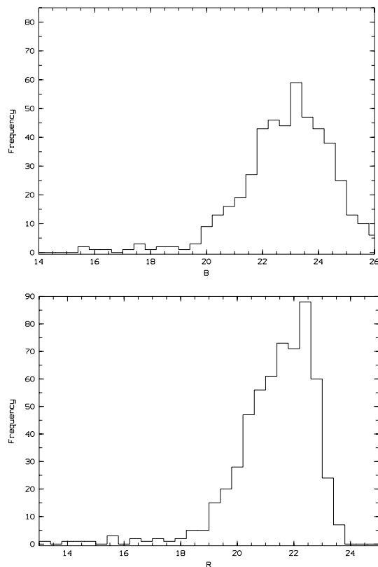
Fig. 3. Magnitude histograms of galaxies along the RX J1119 line of sight. Top: B band, bottom: R band.
