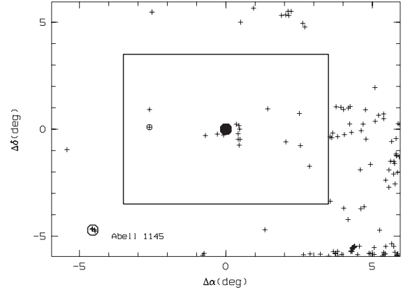
Fig. 1. Map of the 12 \times 12 \text{ deg}^2 area around RX J1119 given in positions relative to the center of RX J1119. The large rectangle is the inner 7 \times 7 \text{ deg}^2 area. Crosses are the galaxies with a redshift in the [0.051, 0.071] redshift range. Inside the 7 \times 7 \text{ deg}^2 area, the only galaxy brighter than the RX J1119 central galaxy by more than 0.2 magnitude is shown as the small circled cross. The position of Abell 1145 is given at the bottom left of the plot. RX J1119 is shown by the central filled circle.
