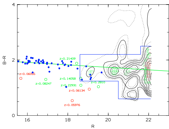
Fig. 5. Total R magnitude versus B-R color for galaxies statistically inside the RX J1119 structure. Galaxies with a known redshift are circles (red: inside the structure, green: outside). Using an adaptive kernel technique, we overlaid the density contours in the R/B-R space. The green line has been normalized to fit the RX J1552 and RX J1416 galaxies in the B-R/R space and to have the Coma cluster slope. Blue dots are galaxies with spectroscopy from the RX J1552 and RX J1416 fossil groups (Mendes de Oliveira et al. 2006, Cypriano et al. 2006) with their magnitudes and colors translated into our system. The blue-delimited area corresponds to our modeling of the positive loci of the density contours. We limit the graph at R \sim 22 to take into account the limited completeness of our catalogs.
