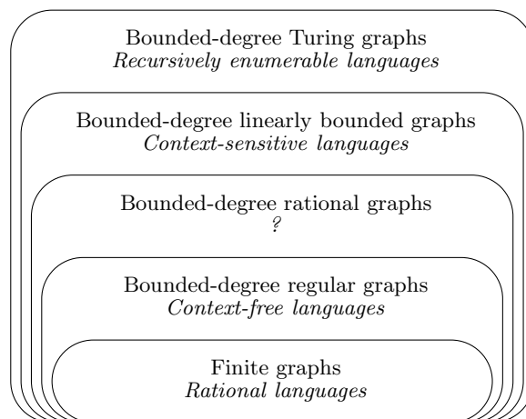
Fig. 11 A Chomsky-like hierarchy of bounded-degree infinite graphs.
