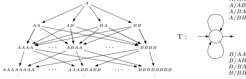
Fig. 7 A finite degree rational graph (together with its transducer) which is not isomorphic to any linearly bounded graph.
