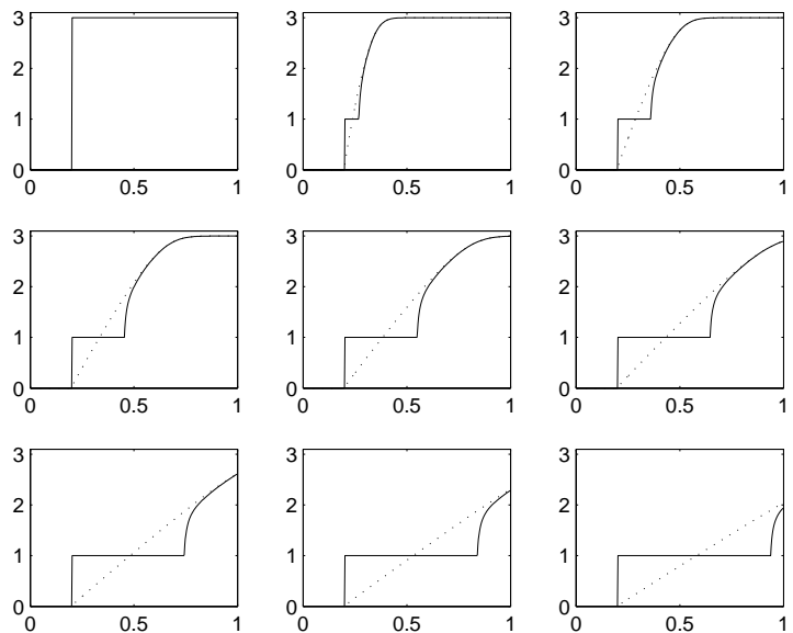
FIGURE 5. Entropy solution u of the Burgers equation with data (B) at different time steps: t = 20 * j * \Delta t ( j = 0, \dots, 8 ). The solution of the discontinuous (resp. continuous) problem is represented with plain (resp. dotted) lines.
