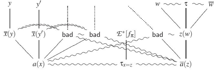
Step 2. (\mathcal{E}_1 \times \mathcal{E}_2)[f_\pi] , where the definition of \mathcal{E}^*[f_\pi] is in Figure 2
