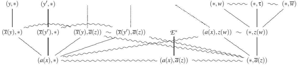
Step 1. \mathcal{E}_1 \times \mathcal{E}_2 , where the definition of \mathcal{E}^* is in Figure 2
