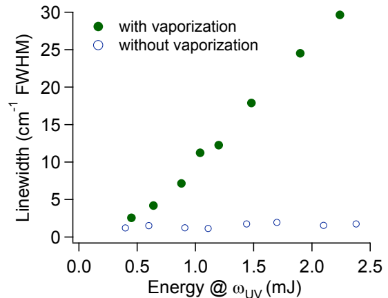
Figure 7 : Linewidth (at half maximum) of VUV signal around the 2-photon resonance vs. energy of the UV beam at 313 \text{ nm} , when the nonlinear interaction takes place in the ablation plume ( full circles ), and in the homogeneous vapor ( open circles ). The excimer fluence on Hg was 0.2 \text{ J}/\text{cm}^2 .
