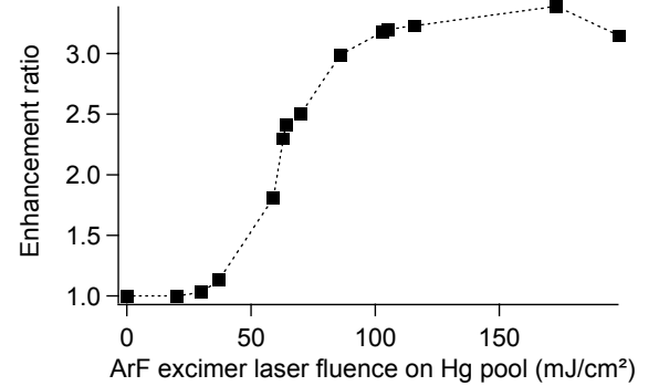
Figure 3 : enhancement of VUV yield versus excimer energy. The excimer spot size on the sample is 1 \text{mm}^2 .
