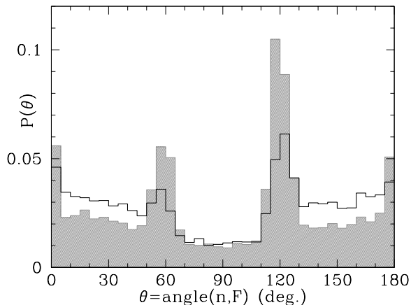
(a) P^* = 0
