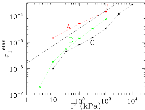
FIG. 12: (Color online) Threshold \epsilon_1^{\text{elas}} above which q differs from E^* \epsilon_1 by more than 5%, versus P , for series A (red), C (black) and D (green). The dashed line has slope 2/3. Data points corresponding to one sample series are connected by thin dotted lines.
