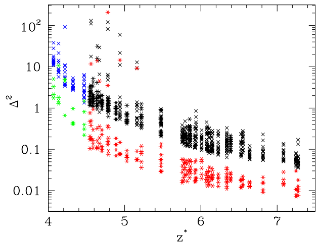
FIG. 4: (Color online) \Delta^2 , as defined in (29), versus backbone coordination number z^* , for isotropic stress increments (red asterisks, green for Z states) and pure deviatoric ones (black crosses, blue for Z states).
