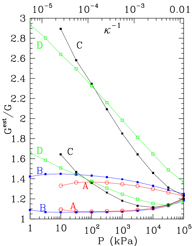
FIG. 5: (Color online) Ratio of estimated to measured values of shear moduli, G^{\text{est}}/G , with G^{\text{est}} = G^{\text{Voigt}} (larger values) and G^{\text{est}} = G^{\text{LRJ}} (smaller values), versus P or \kappa^{-1} , in sample series A (red), B (blue), C (black) and D (green).
