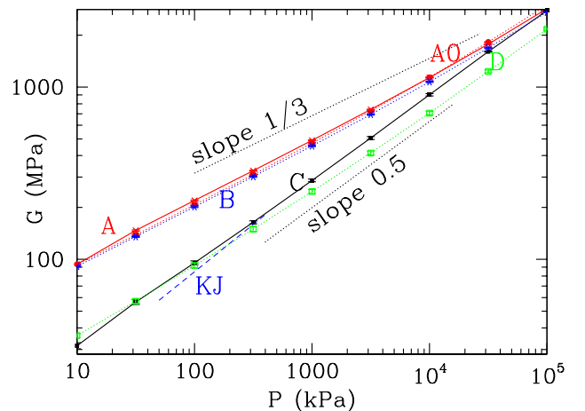
(b) G versus P
