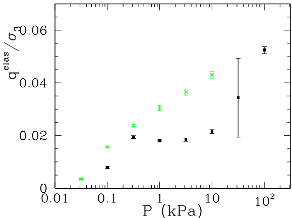
FIG. 14: (Color online) Stress ratio q^{\text{elas}}/P above which q/E differs from \epsilon_1 by more than 5%, versus P , for series C (black, lower data points) and D (green).
