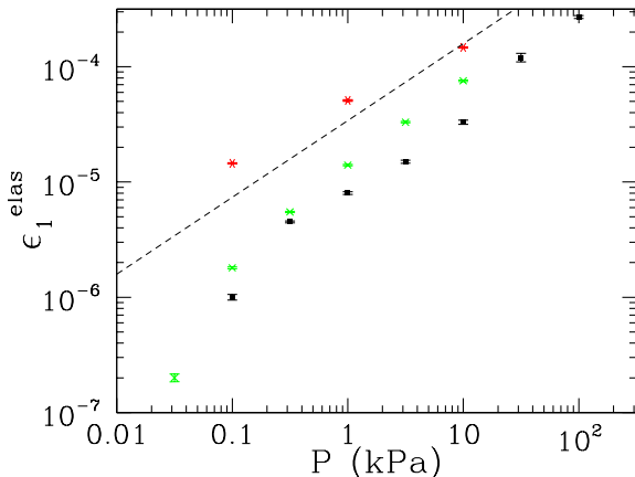
FIG. 12: (Color online) Threshold \epsilon_1^{\text{elas}} above which q differs from E\epsilon_1 by more than 5%, versus P , for series A (red), C (black) and D (green). The dotted line has slope 2/3 .
