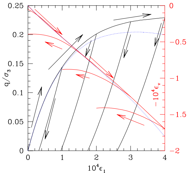
FIG. 15: (Color online) Deviator stress (black, left axis) and volumetric strain (red, right axis) versus axial strain in triaxial compression for small strains, with unloading curves, in a D sample initially under P=100 kPa. The blue dotted curves show the results of a calculation with the sole contacts that are initially present.
