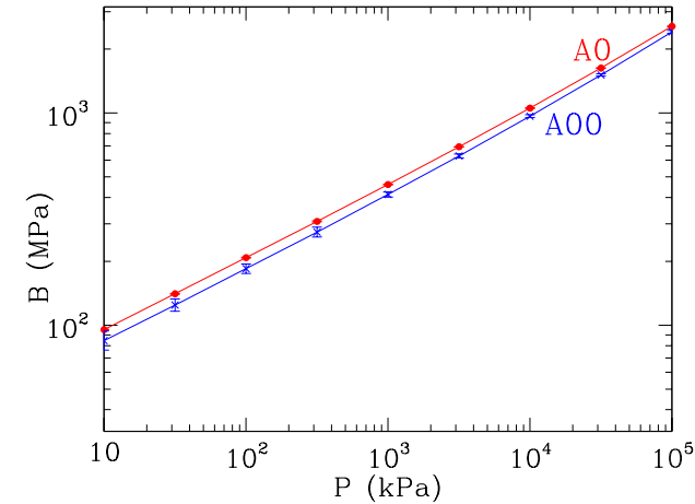
(a) Bulk modulus.
