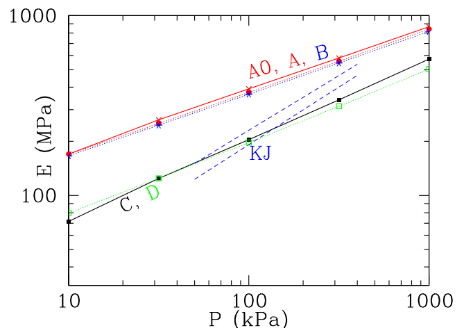
FIG. 10: (Color online) Young modulus in numerical samples A, A0, B, C, D, labelled with same colors and symbols as on Fig. 9, compared to fits through data points of Kuwano and Jardine (dotted lines, KJ) [6], with two sets of values because of fabric anisotropy.
