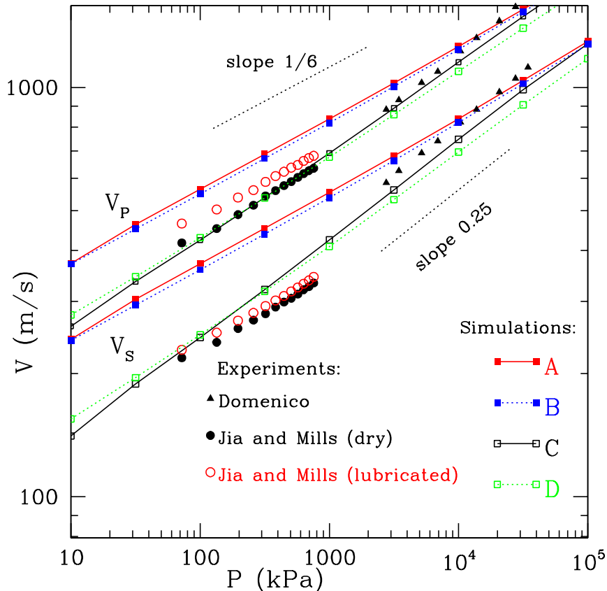
FIG. 9: (Color online) Sound velocities V_P and V_S versus confining pressure P on double logarithmic plot for the experimental dry (vibrated) and lubricated samples of Jia and Mills, and of Domenico, to which numerical values for simulated states A, B, C and D are compared.
