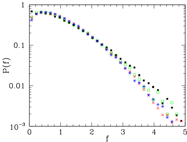
FIG. 11: (Color online) Distribution of normal forces, normalized by its average, f = \frac{N}{\langle N \rangle} , in states A (red crosses), B (blue asterisks), C (black square dots) and D (green open squares) at the lowest simulated pressure.
