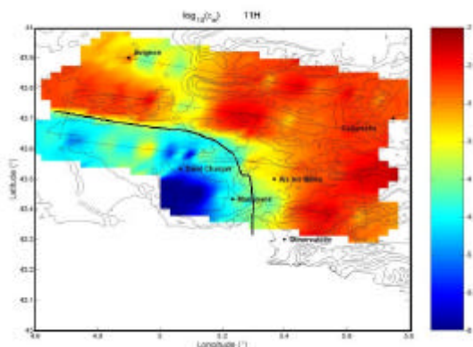
Fig. 1 : Horizontal field of the dissipation coefficient of turbulent kinetic energy ( \epsilon ) measured at 11UTC on June 26. The black line delineates the area inside the BL (red and yellow) from the outside (blue).
