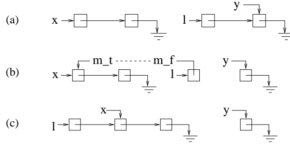
Fig. 2. An example store, the store after the statement l \rightarrow \text{next} = x , and after a rearrangement
