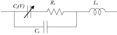
Fig. 9. Macom MA4ST-1240 Varactor equivalent electrical circuit.
