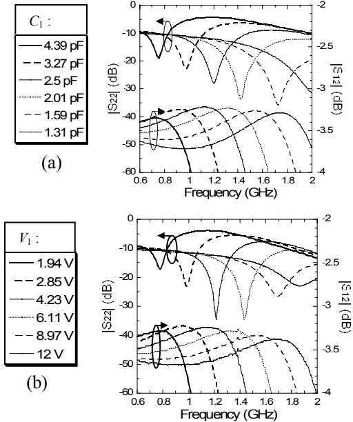
Fig. 13. |S_{22}| and |S_{12}| . (a) Simulations. (b) Measurements.
