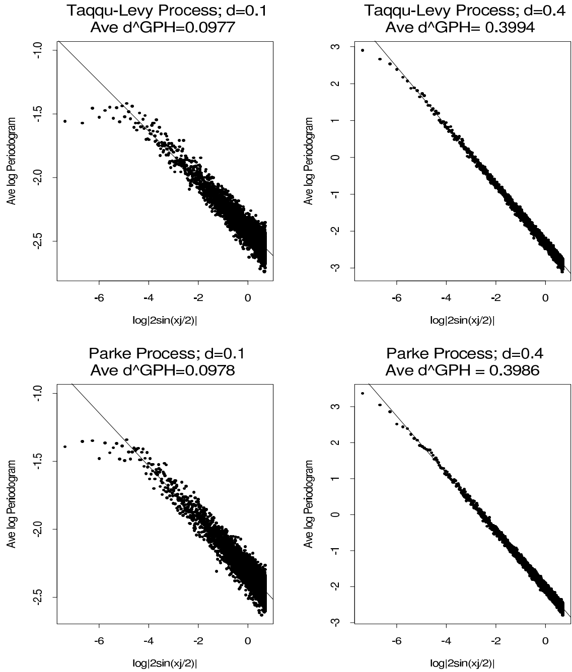
Figure 6: Scatterplots of Average Log Periodogram vs. \log |2 \sin(x_j/2)| ; j=1,2,\dots,4999
