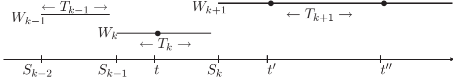
Figure 2: A path ( \bullet ) of the renewal-reward process: X_t = W_k , X_{t'} = X_{t''} = W_{k+1} .
