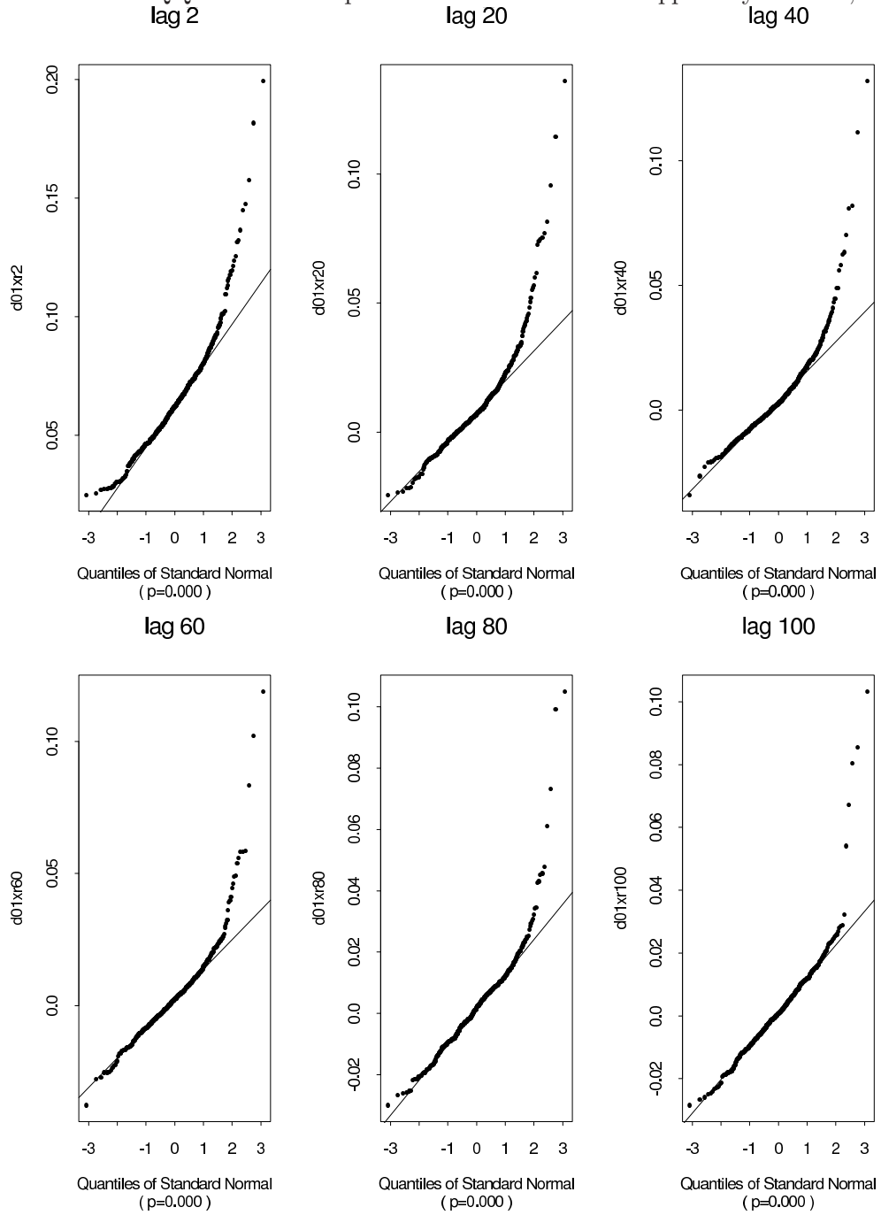
Figure 7: Normal QQ Plots of Sample Autocorrelations for Taqqu-Levy Process, d=0.1
