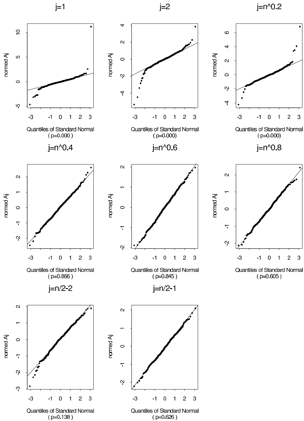
Figure 3: QQ Plots of the Normalized Fourier Cosine Coefficients A_j/f(\omega_j)^{\frac{1}{2}} for Parke process; n=10000 , d=0.1
