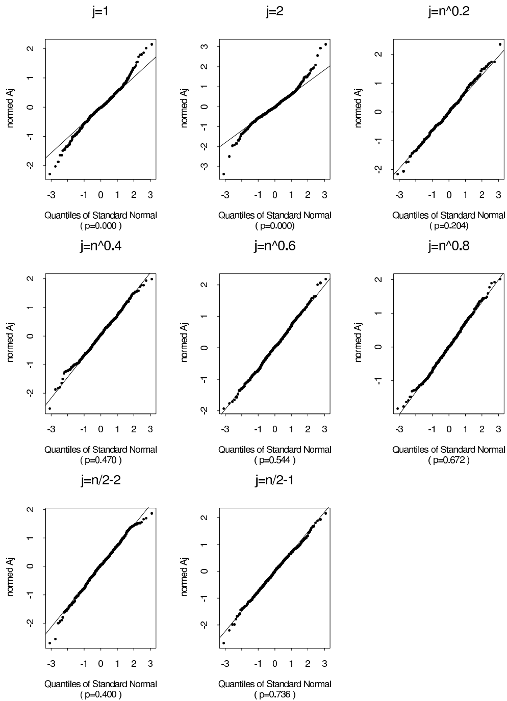
Figure 4: QQ Plots of the Normalized Fourier Cosine Coefficients A_j/f(\omega_j)^{\frac{1}{2}} for Parke process; n=10000 , d=0.4
