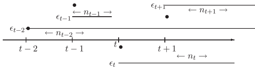
Figure 1: A path ( \bullet ) of the error duration process: X_t = \epsilon_{t-2} + \epsilon_t , X_{t+1} = \epsilon_{t-2} + \epsilon_t + \epsilon_{t+1} .
