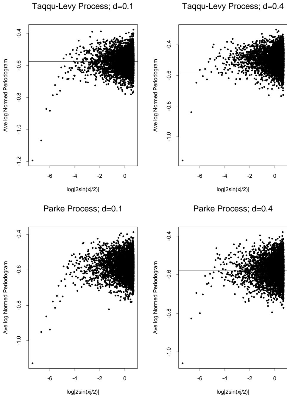
Figure 5: Scatterplots of Average Log Normalized Periodogram vs. \log|2\sin(x_j/2)| ; j=1,2,\dots,4999 . Horizontal line represents -\gamma = -0.577216 .
