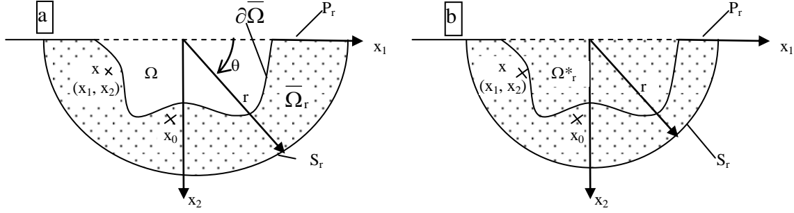
Figure 1 a: Integration domain \bar{\Omega}_R (in grey) b: auxiliary integration domain \Omega_r^*
